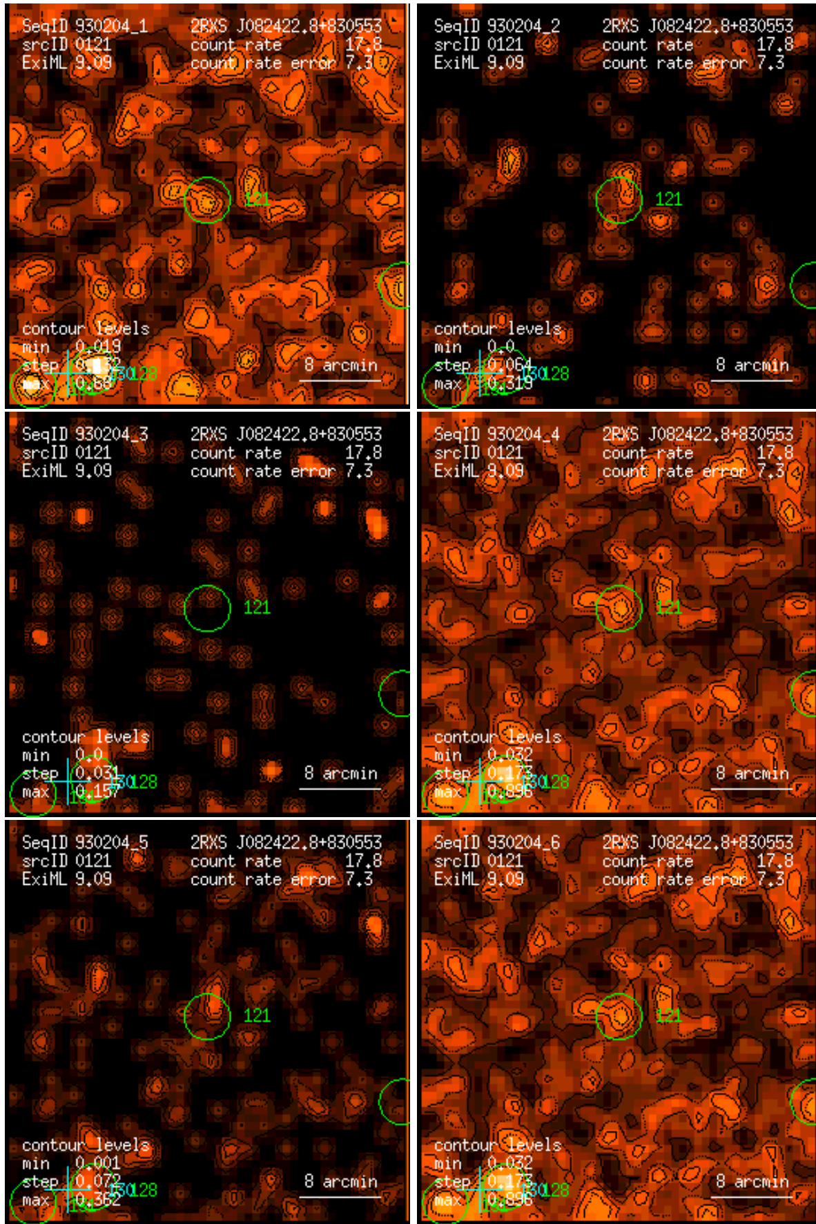
Figure 121: RASS 930204: detection 0121: band rate images, Gaussian filter: (1) PSPC channels 11 – 41, (2) 52 – 90, (3) 91 – 201, (4) 11 – 235, (5) 52 – 201, (6) 11 – 201. Broad band rates in counts/ks. Band rate contour levels in counts/ks/arcmin 2 .
