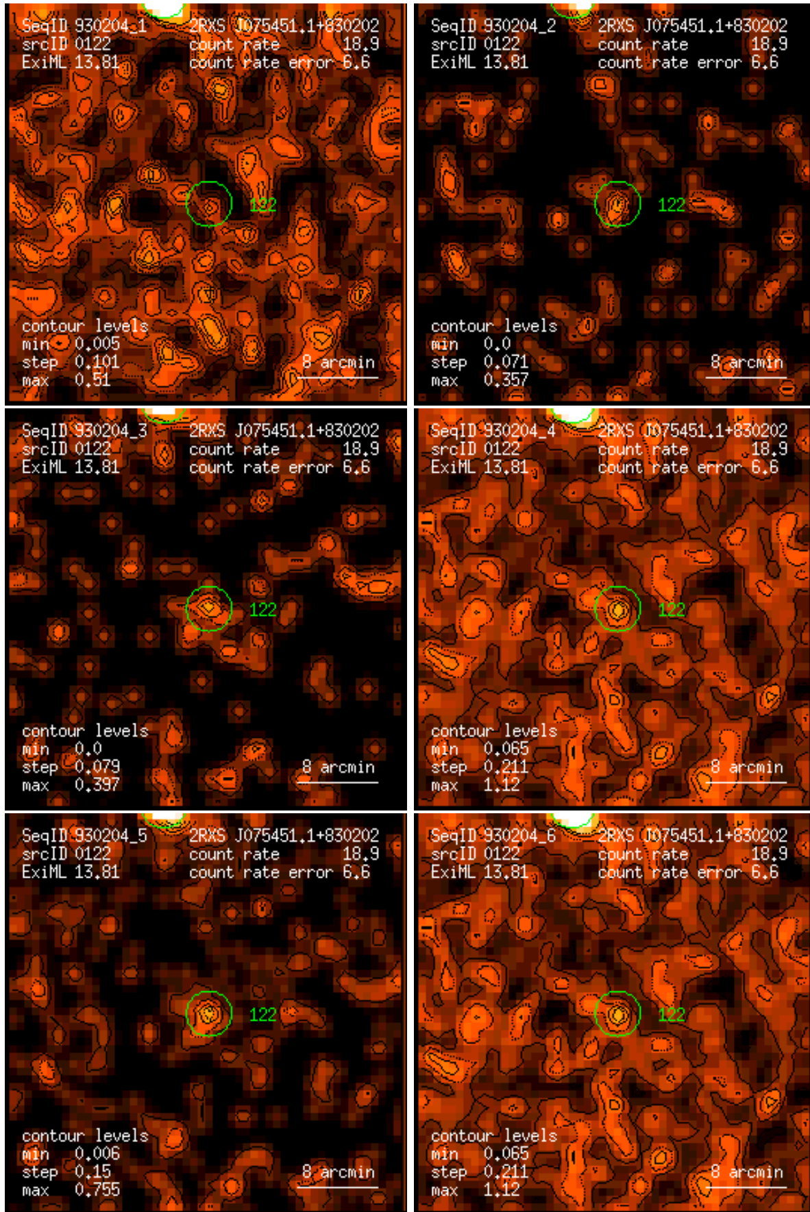
Figure 122: RASS 930204: detection 0122: band rate images, Gaussian filter: (1) PSPC channels 11 – 41, (2) 52 – 90, (3) 91 – 201, (4) 11 – 235, (5) 52 – 201, (6) 11 – 201. Broad band rates in counts/ks. Band rate contour levels in counts/ks/arcmin 2 .
