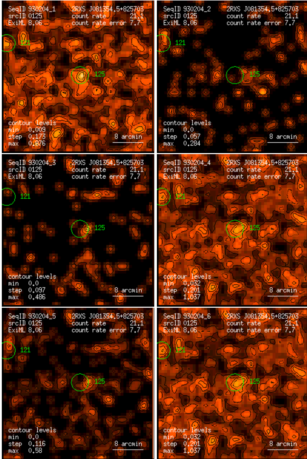
Figure 125: RASS 930204: detection 0125: band rate images, Gaussian filter: (1) PSPC channels 11 – 41, (2) 52 – 90, (3) 91 – 201, (4) 11 – 235, (5) 52 – 201, (6) 11 – 201. Broad band rates in counts/ks. Band rate contour levels in counts/ks/arcmin 2 .
