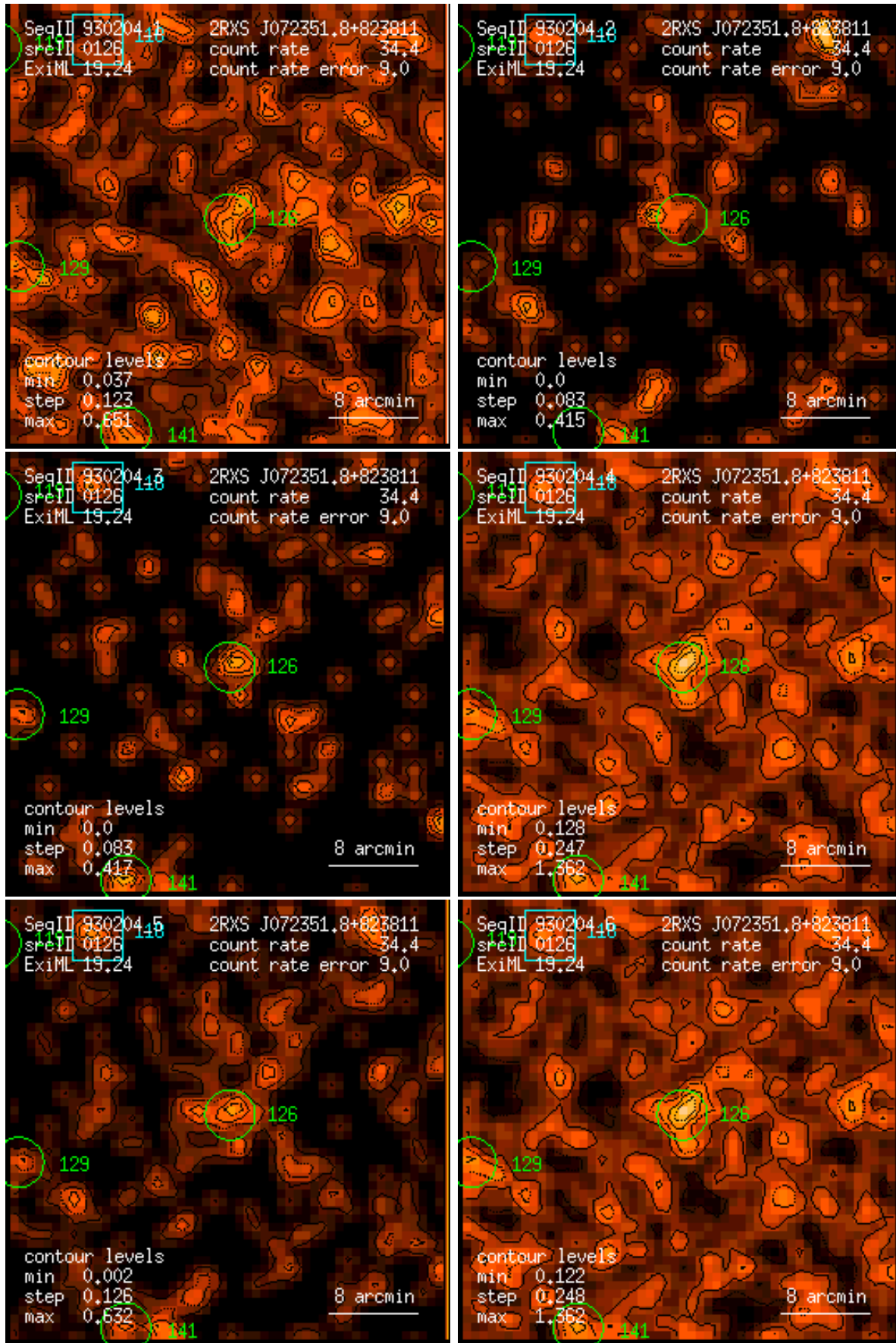
Figure 126: RASS 930204: detection 0126: band rate images, Gaussian filter: (1) PSPC channels 11 – 41, (2) 52 – 90, (3) 91 – 201, (4) 11 – 235, (5) 52 – 201, (6) 11 – 201. Broad band rates in counts/ks. Band rate contour levels in counts/ks/arcmin 2 .
