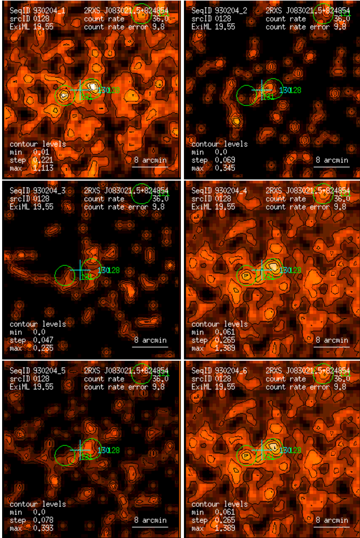
Figure 128: RASS 930204: detection 0128: band rate images, Gaussian filter: (1) PSPC channels 11 – 41, (2) 52 – 90, (3) 91 – 201, (4) 11 – 235, (5) 52 – 201, (6) 11 – 201. Broad band rates in counts/ks. Band rate contour levels in counts/ks/arcmin 2 .
