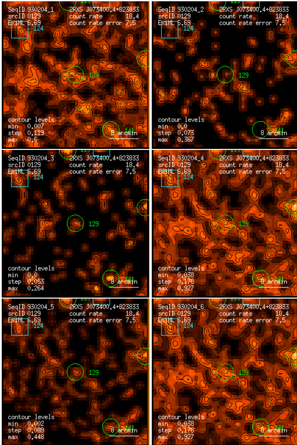
Figure 129: RASS 930204: detection 0129: band rate images, Gaussian filter: (1) PSPC channels 11 – 41, (2) 52 – 90, (3) 91 – 201, (4) 11 – 235, (5) 52 – 201, (6) 11 – 201. Broad band rates in counts/ks. Band rate contour levels in counts/ks/arcmin 2 .
