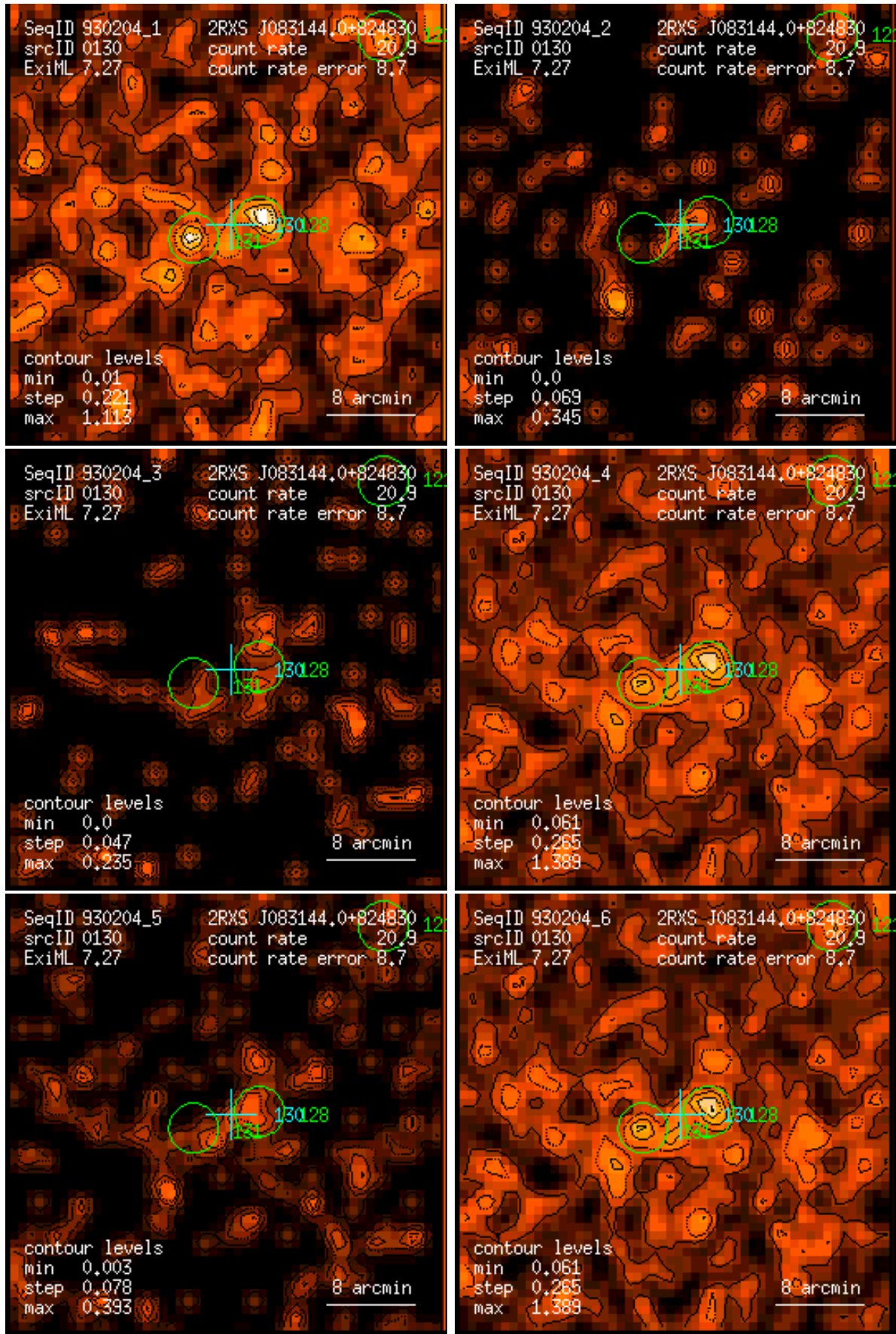
Figure 130: RASS 930204: detection 0130: band rate images, Gaussian filter: (1) PSPC channels 11 – 41, (2) 52 – 90, (3) 91 – 201, (4) 11 – 235, (5) 52 – 201, (6) 11 – 201. Broad band rates in counts/ks. Band rate contour levels in counts/ks/arcmin 2 .
