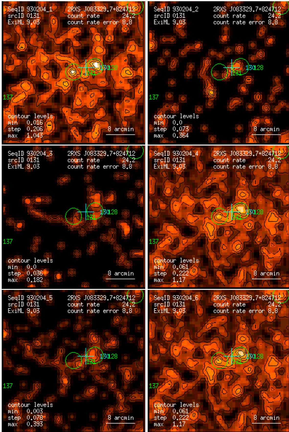
Figure 131: RASS 930204: detection 0131: band rate images, Gaussian filter: (1) PSPC channels 11 – 41, (2) 52 – 90, (3) 91 – 201, (4) 11 – 235, (5) 52 – 201, (6) 11 – 201. Broad band rates in counts/ks. Band rate contour levels in counts/ks/arcmin 2 .
