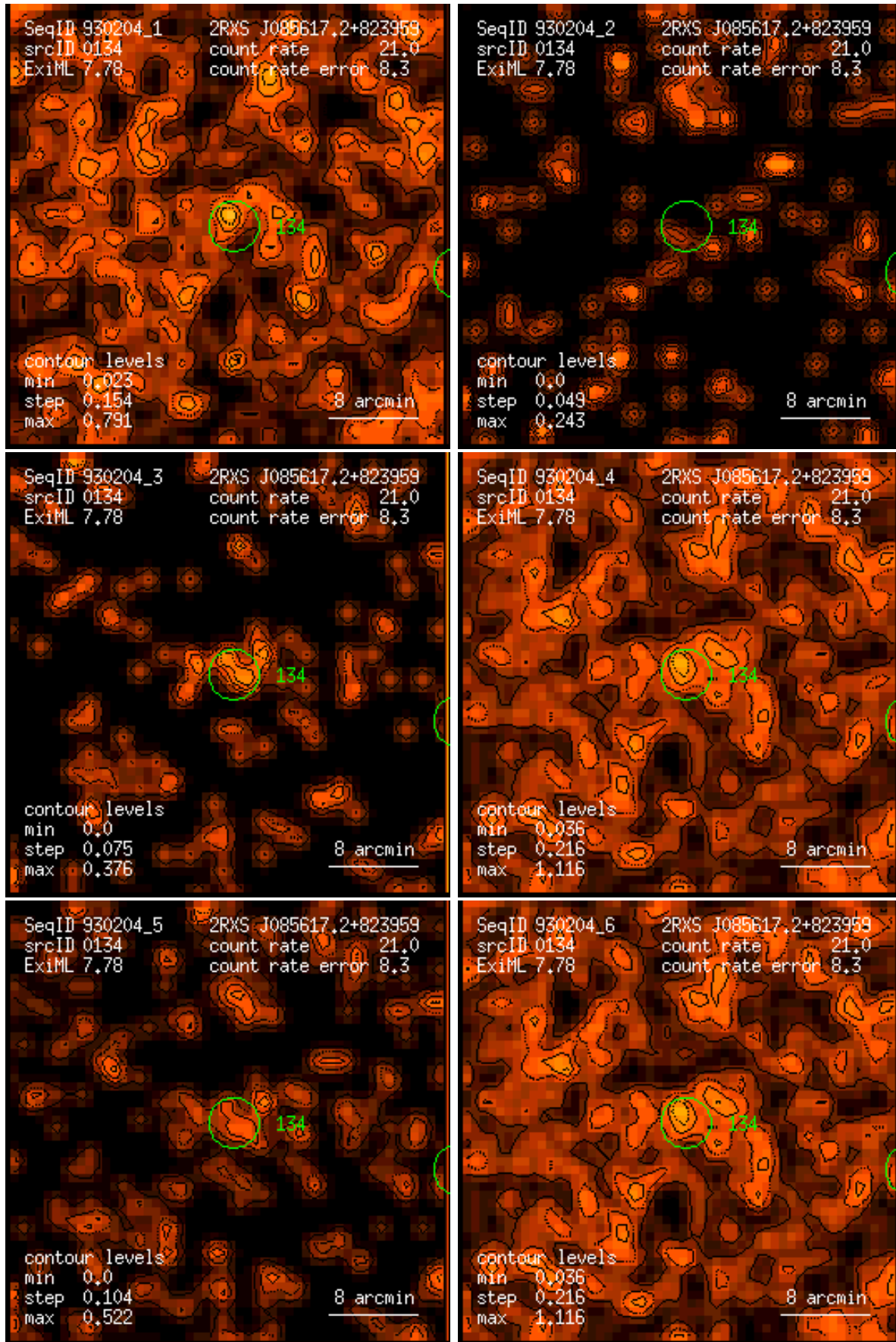
Figure 134: RASS 930204: detection 0134: band rate images, Gaussian filter: (1) PSPC channels 11 – 41, (2) 52 – 90, (3) 91 – 201, (4) 11 – 235, (5) 52 – 201, (6) 11 – 201. Broad band rates in counts/ks. Band rate contour levels in counts/ks/arcmin 2 .
