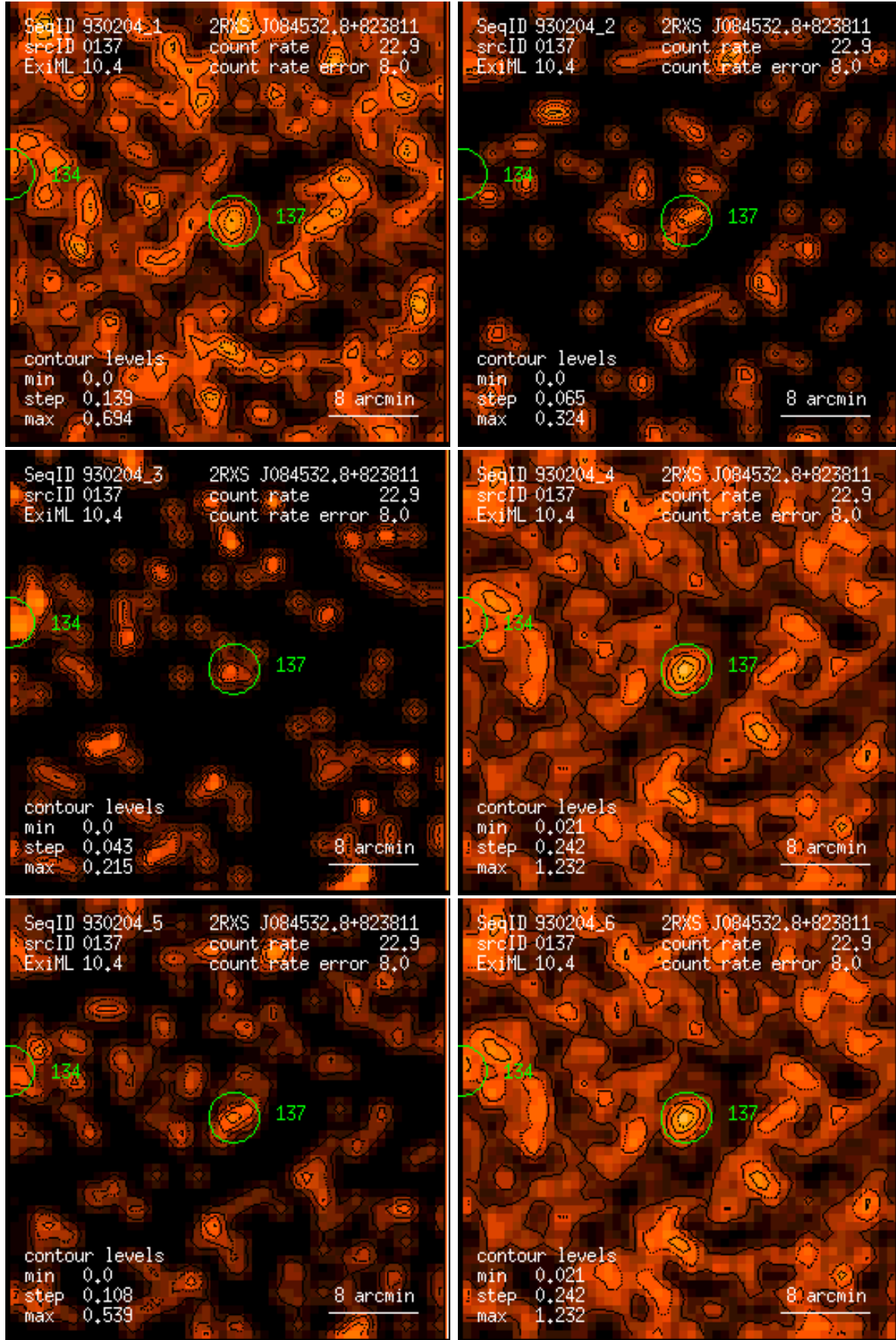
Figure 137: RASS 930204: detection 0137: band rate images, Gaussian filter: (1) PSPC channels 11 – 41, (2) 52 – 90, (3) 91 – 201, (4) 11 – 235, (5) 52 – 201, (6) 11 – 201. Broad band rates in counts/ks. Band rate contour levels in counts/ks/arcmin 2 .
