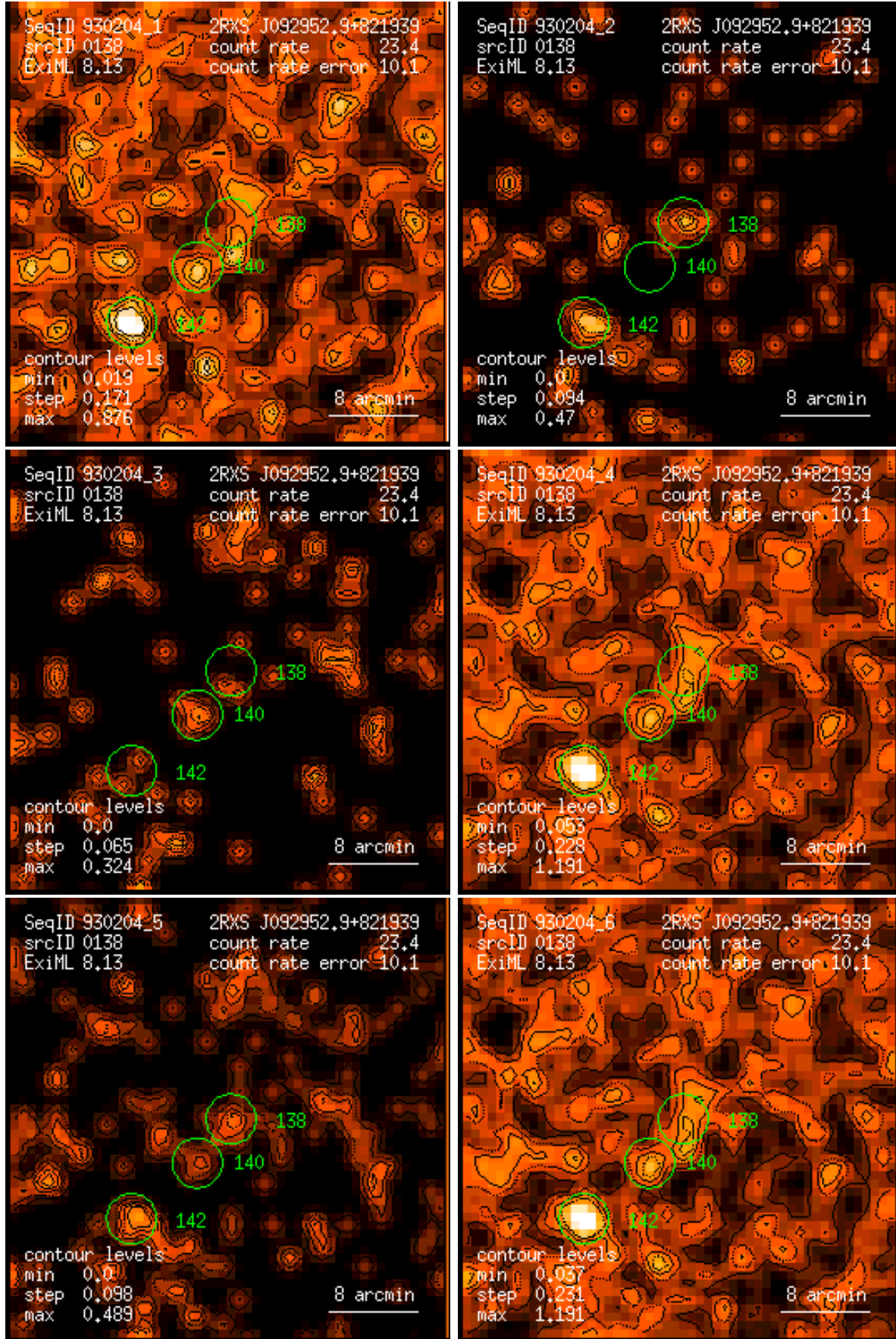
Figure 138: RASS 930204: detection 0138: band rate images, Gaussian filter: (1) PSPC channels 11 – 41, (2) 52 – 90, (3) 91 – 201, (4) 11 – 235, (5) 52 – 201, (6) 11 – 201. Broad band rates in counts/ks. Band rate contour levels in counts/ks/arcmin 2 .
