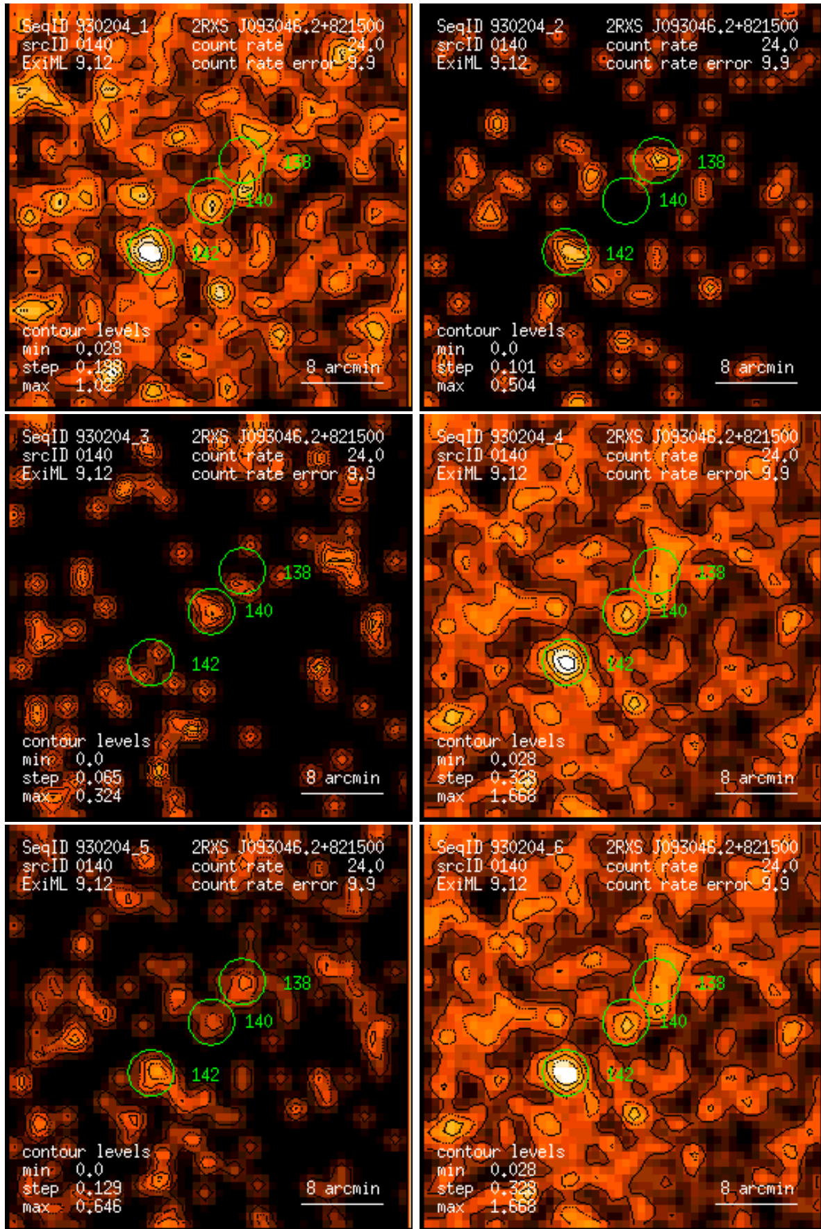
Figure 140: RASS 930204: detection 0140: band rate images, Gaussian filter: (1) PSPC channels 11 – 41, (2) 52 – 90, (3) 91 – 201, (4) 11 – 235, (5) 52 – 201, (6) 11 – 201. Broad band rates in counts/ks. Band rate contour levels in counts/ks/arcmin 2 .
