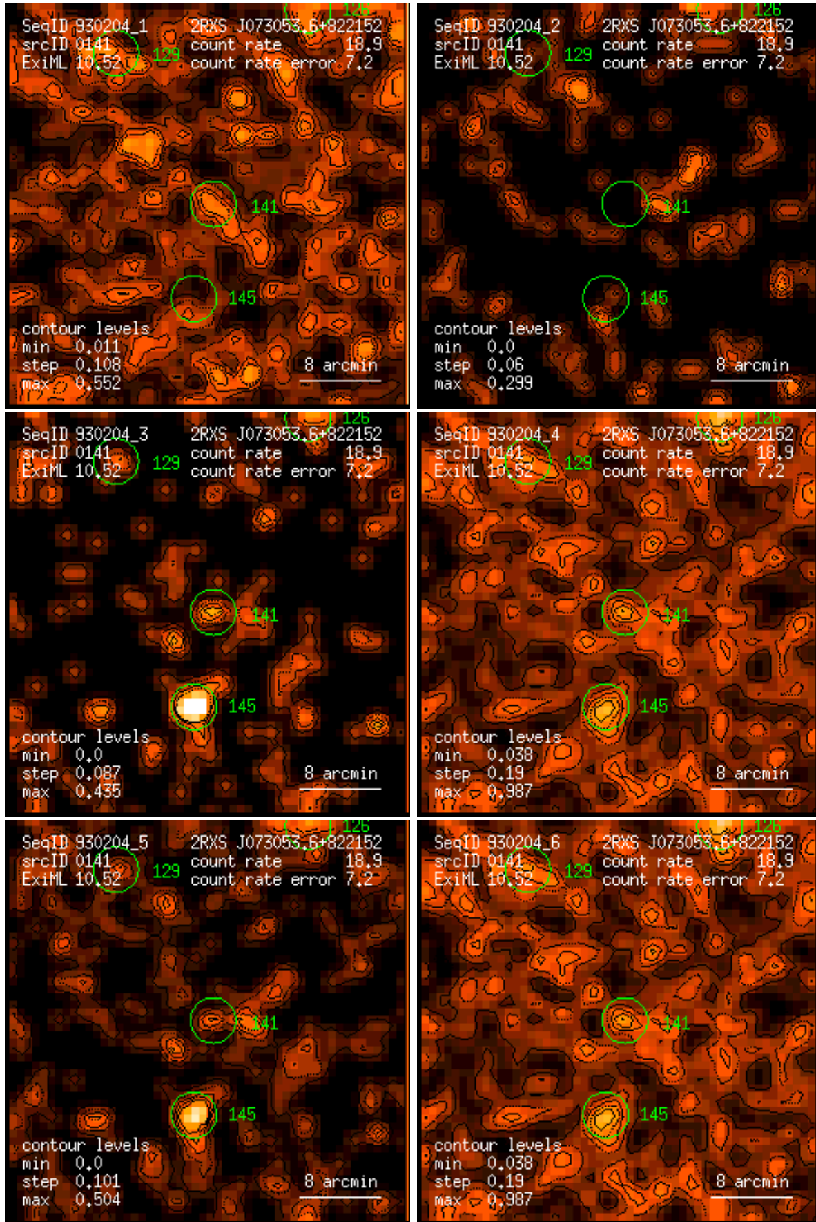
Figure 141: RASS 930204: detection 0141: band rate images, Gaussian filter: (1) PSPC channels 11 – 41, (2) 52 – 90, (3) 91 – 201, (4) 11 – 235, (5) 52 – 201, (6) 11 – 201. Broad band rates in counts/ks. Band rate contour levels in counts/ks/arcmin 2 .
