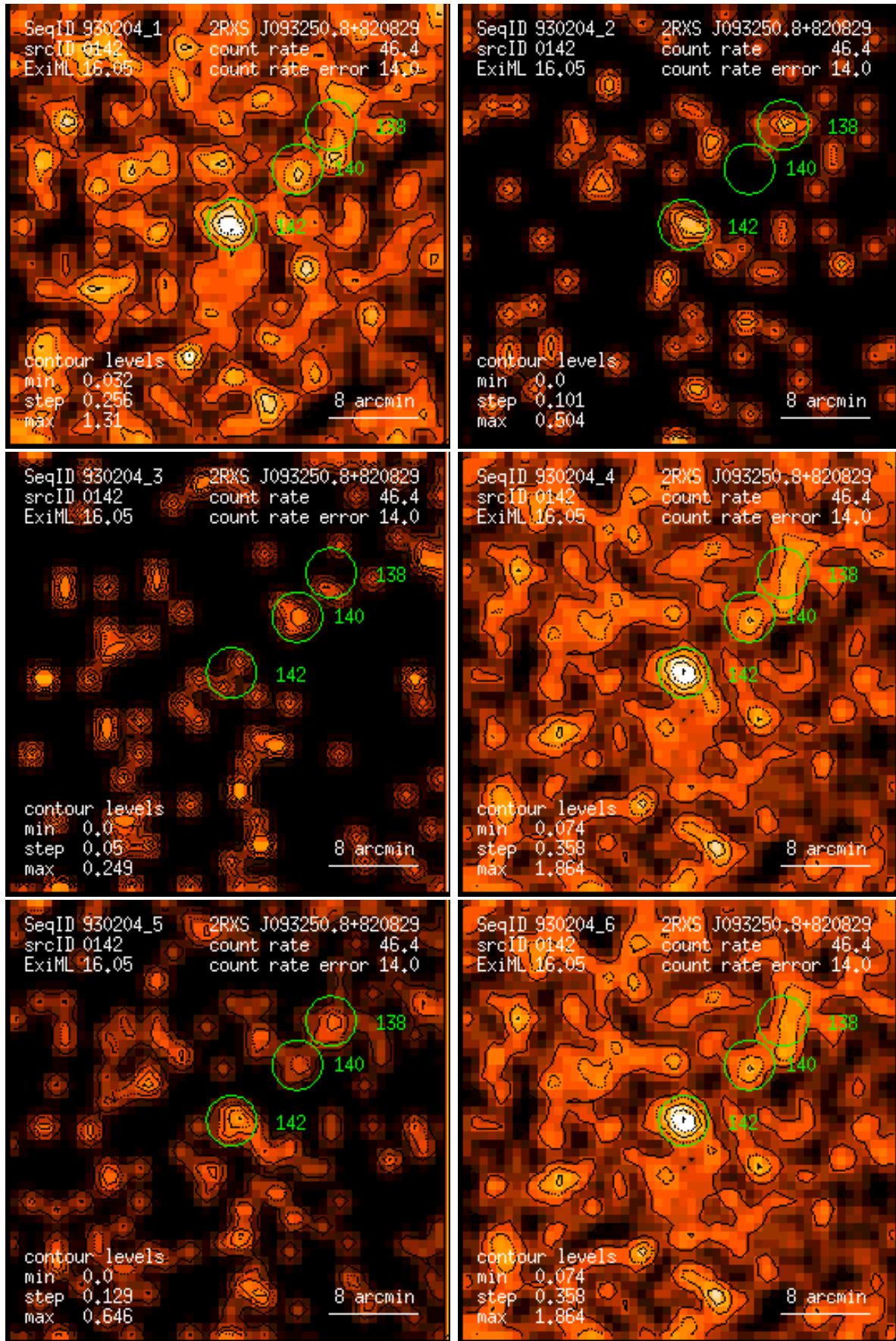
Figure 142: RASS 930204: detection 0142: band rate images, Gaussian filter: (1) PSPC channels 11 – 41, (2) 52 – 90, (3) 91 – 201, (4) 11 – 235, (5) 52 – 201, (6) 11 – 201. Broad band rates in counts/ks. Band rate contour levels in counts/ks/arcmin 2 .
