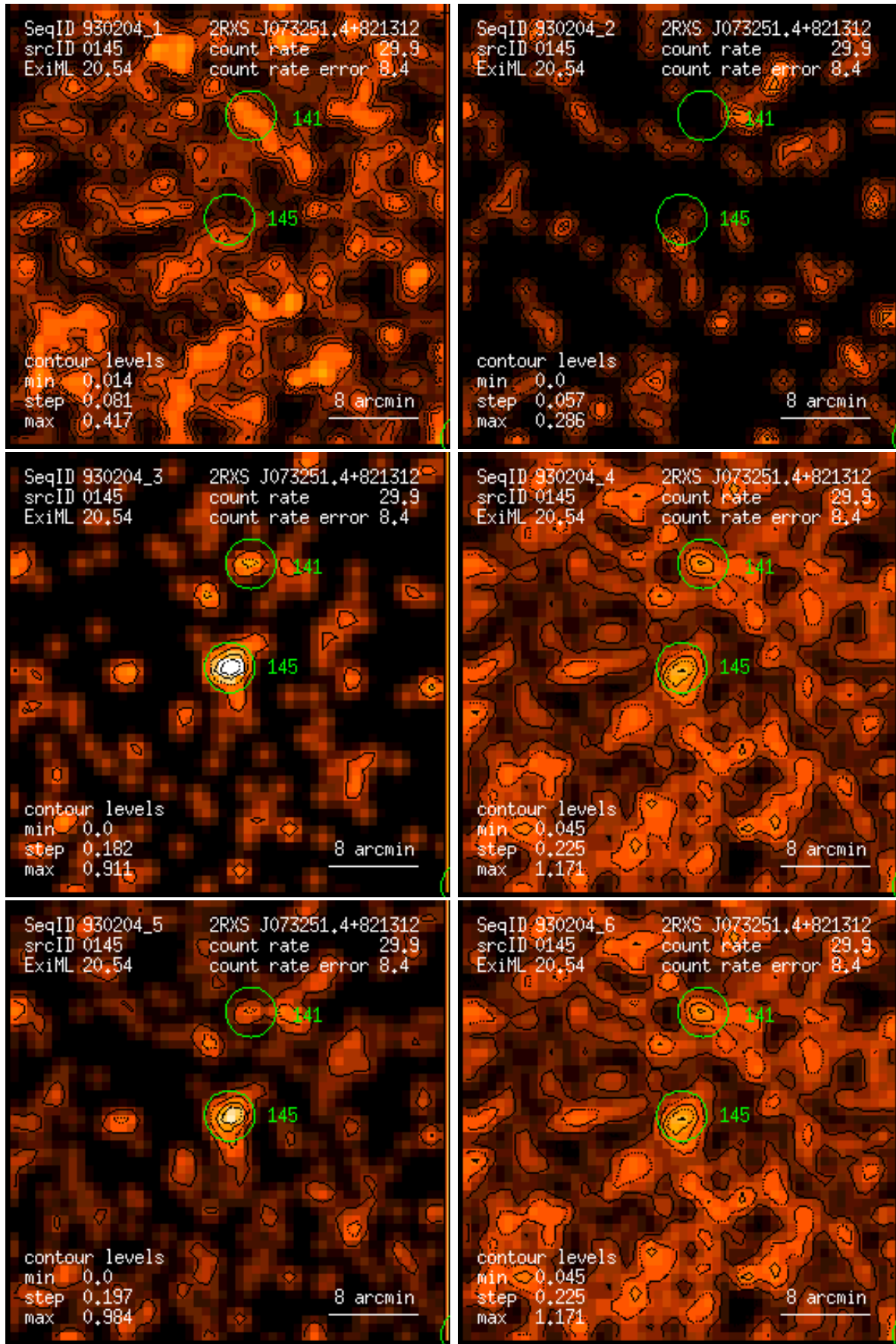
Figure 145: RASS 930204: detection 0145: band rate images, Gaussian filter: (1) PSPC channels 11 – 41, (2) 52 – 90, (3) 91 – 201, (4) 11 – 235, (5) 52 – 201, (6) 11 – 201. Broad band rates in counts/ks. Band rate contour levels in counts/ks/arcmin 2 .
