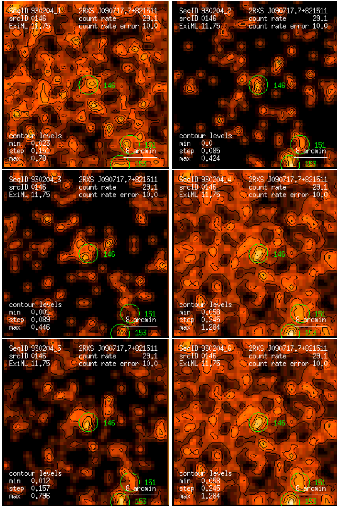
Figure 146: RASS 930204: detection 0146: band rate images, Gaussian filter: (1) PSPC channels 11 – 41, (2) 52 – 90, (3) 91 – 201, (4) 11 – 235, (5) 52 – 201, (6) 11 – 201. Broad band rates in counts/ks. Band rate contour levels in counts/ks/arcmin 2 .
