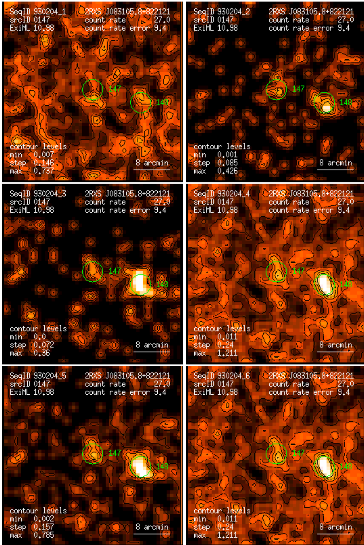
Figure 147: RASS 930204: detection 0147: band rate images, Gaussian filter: (1) PSPC channels 11 – 41, (2) 52 – 90, (3) 91 – 201, (4) 11 – 235, (5) 52 – 201, (6) 11 – 201. Broad band rates in counts/ks. Band rate contour levels in counts/ks/arcmin 2 .
