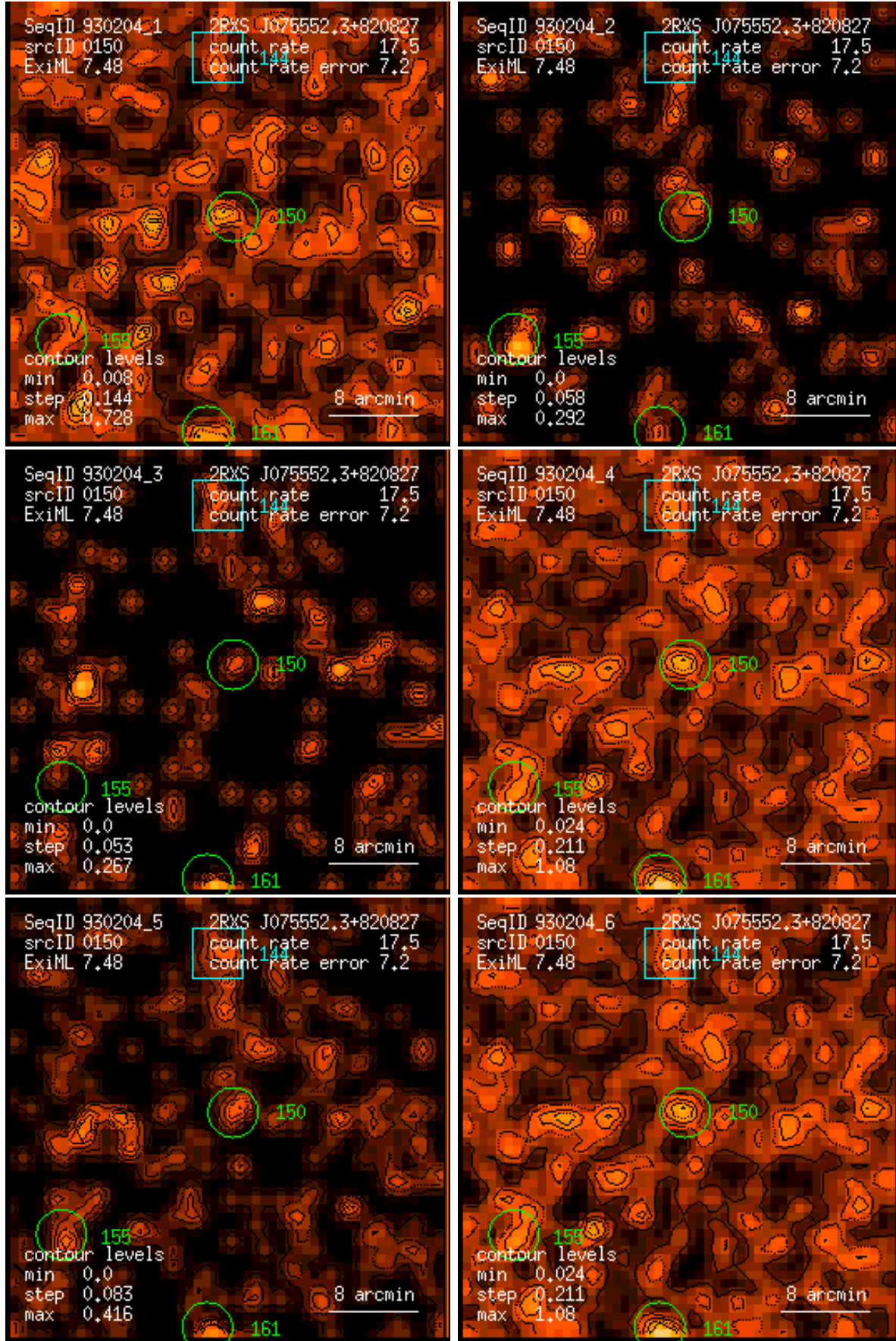
Figure 150: RASS 930204: detection 0150: band rate images, Gaussian filter: (1) PSPC channels 11 – 41, (2) 52 – 90, (3) 91 – 201, (4) 11 – 235, (5) 52 – 201, (6) 11 – 201. Broad band rates in counts/ks. Band rate contour levels in counts/ks/arcmin 2 .
