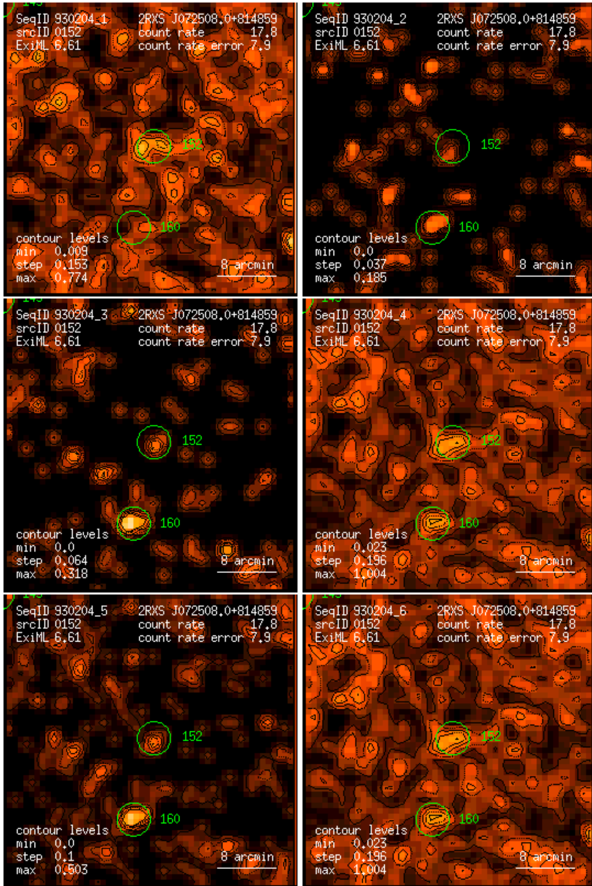
Figure 152: RASS 930204: detection 0152: band rate images, Gaussian filter: (1) PSPC channels 11 – 41, (2) 52 – 90, (3) 91 – 201, (4) 11 – 235, (5) 52 – 201, (6) 11 – 201. Broad band rates in counts/ks. Band rate contour levels in counts/ks/arcmin 2 .
