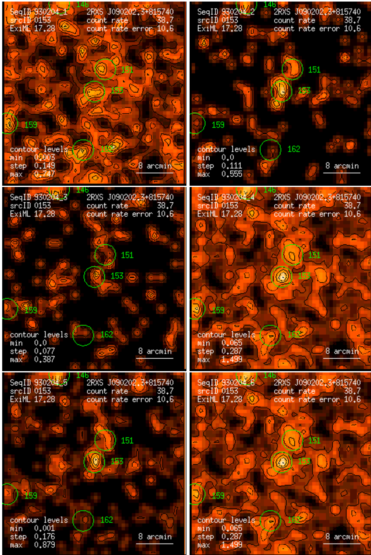
Figure 153: RASS 930204: detection 0153: band rate images, Gaussian filter: (1) PSPC channels 11 – 41, (2) 52 – 90, (3) 91 – 201, (4) 11 – 235, (5) 52 – 201, (6) 11 – 201. Broad band rates in counts/ks. Band rate contour levels in counts/ks/arcmin 2 .
