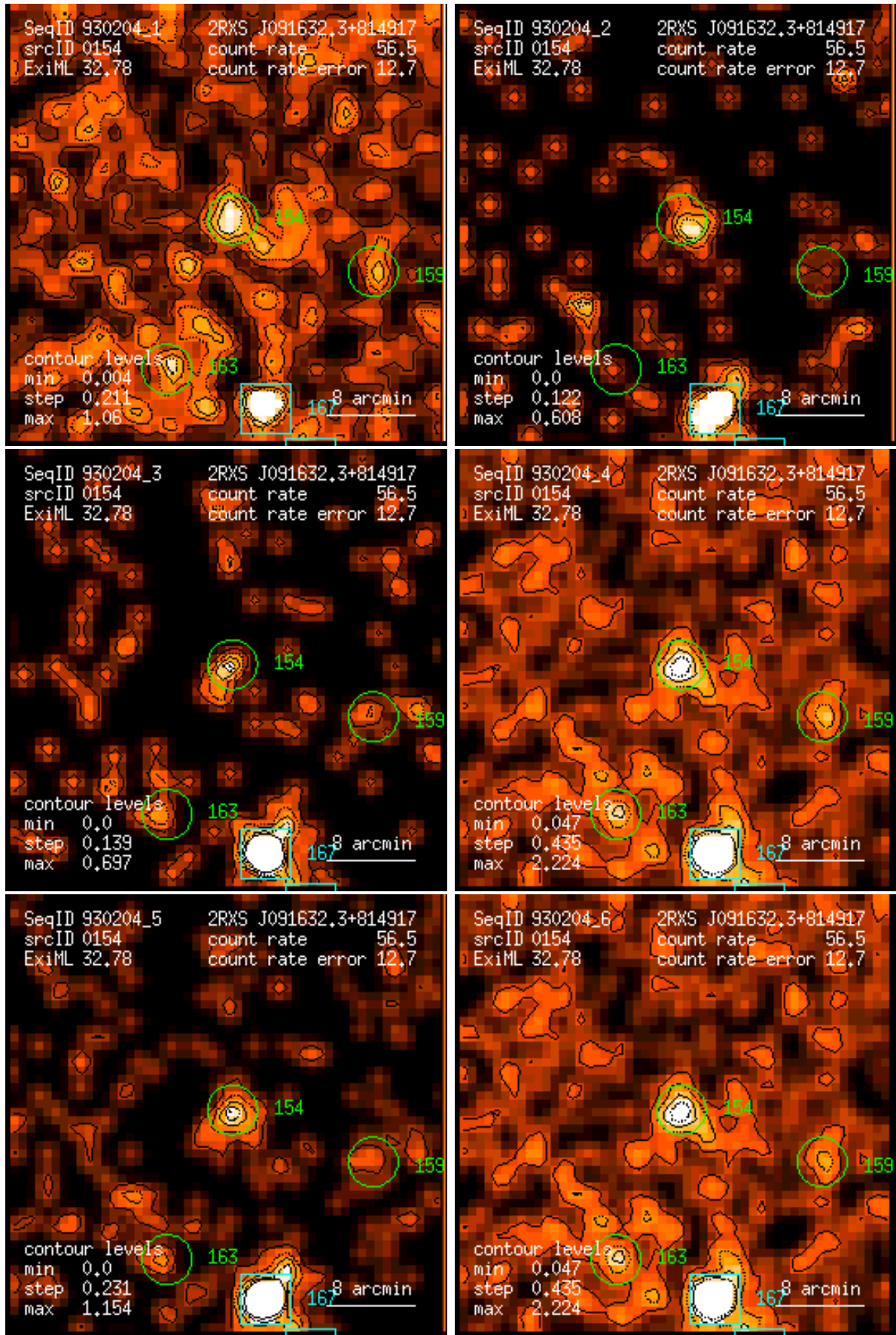
Figure 154: RASS 930204: detection 0154: band rate images, Gaussian filter: (1) PSPC channels 11 – 41, (2) 52 – 90, (3) 91 – 201, (4) 11 – 235, (5) 52 – 201, (6) 11 – 201. Broad band rates in counts/ks. Band rate contour levels in counts/ks/arcmin 2 .
