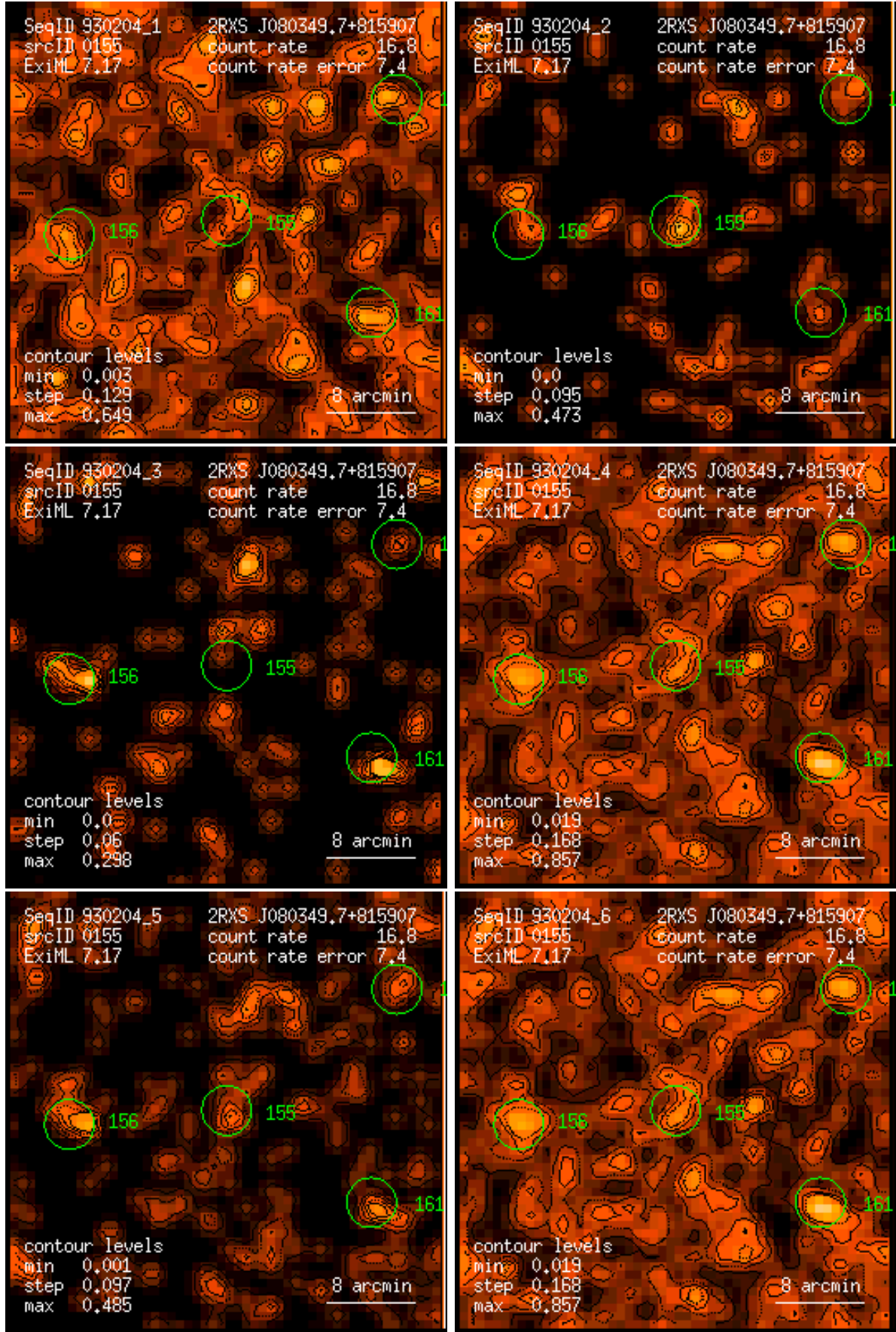
Figure 155: RASS 930204: detection 0155: band rate images, Gaussian filter: (1) PSPC channels 11 – 41, (2) 52 – 90, (3) 91 – 201, (4) 11 – 235, (5) 52 – 201, (6) 11 – 201. Broad band rates in counts/ks. Band rate contour levels in counts/ks/arcmin 2 .
