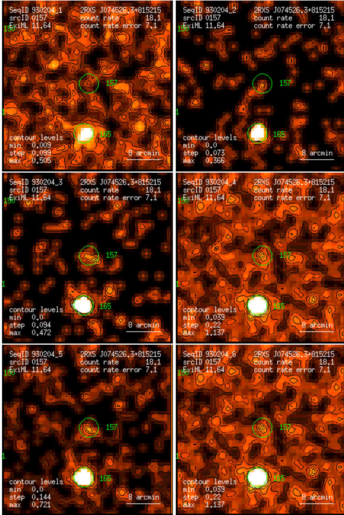
Figure 157: RASS 930204: detection 0157: band rate images, Gaussian filter: (1) PSPC channels 11 – 41, (2) 52 – 90, (3) 91 – 201, (4) 11 – 235, (5) 52 – 201, (6) 11 – 201. Broad band rates in counts/ks. Band rate contour levels in counts/ks/arcmin 2 .
