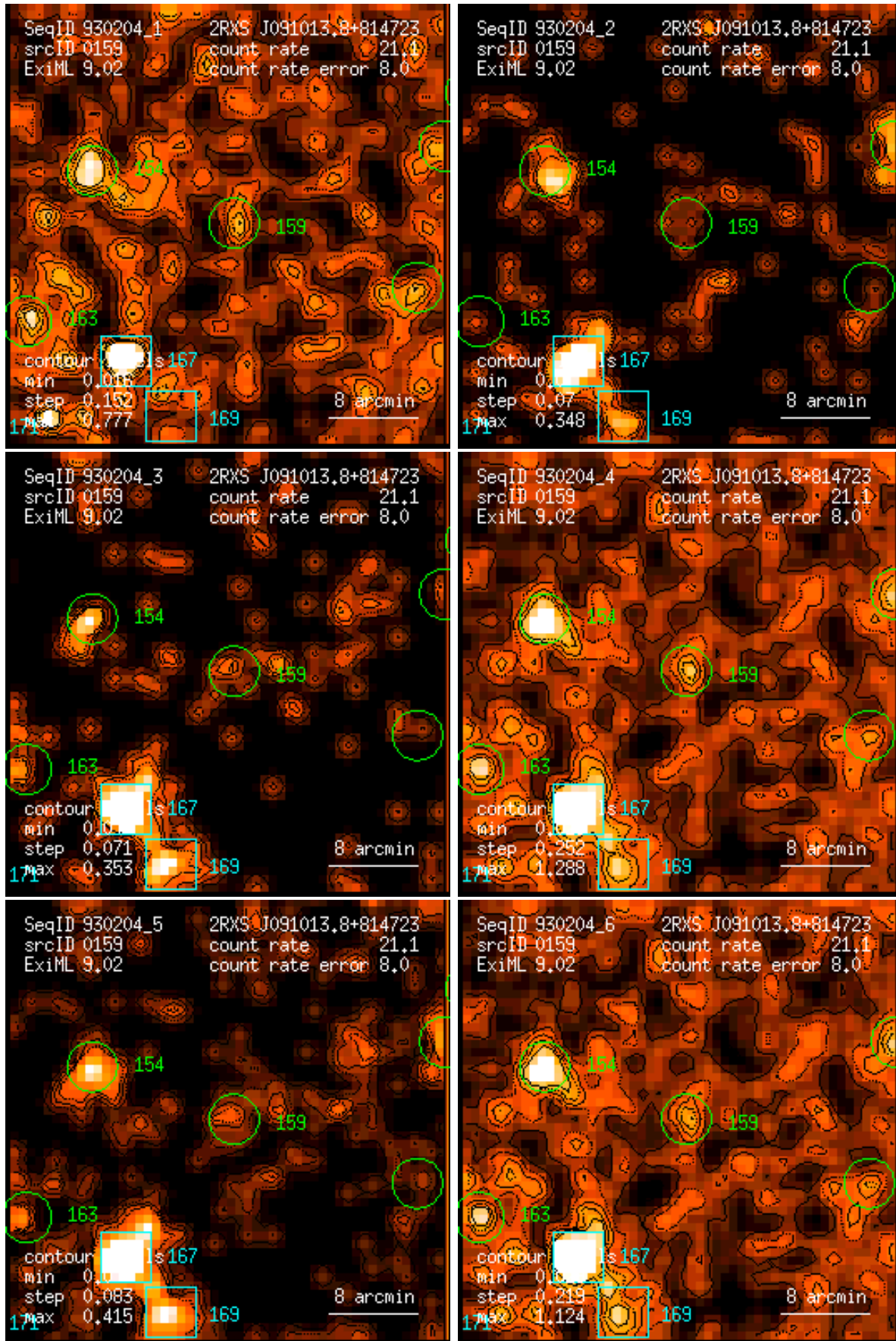
Figure 159: RASS 930204: detection 0159: band rate images, Gaussian filter: (1) PSPC channels 11 – 41, (2) 52 – 90, (3) 91 – 201, (4) 11 – 235, (5) 52 – 201, (6) 11 – 201. Broad band rates in counts/ks. Band rate contour levels in counts/ks/arcmin 2 .
