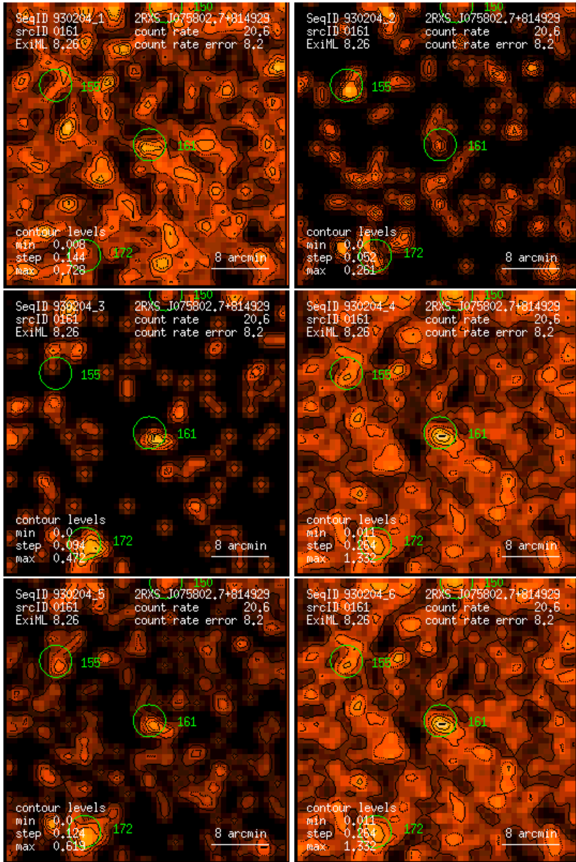
Figure 161: RASS 930204: detection 0161: band rate images, Gaussian filter: (1) PSPC channels 11 – 41, (2) 52 – 90, (3) 91 – 201, (4) 11 – 235, (5) 52 – 201, (6) 11 – 201. Broad band rates in counts/ks. Band rate contour levels in counts/ks/arcmin 2 .
