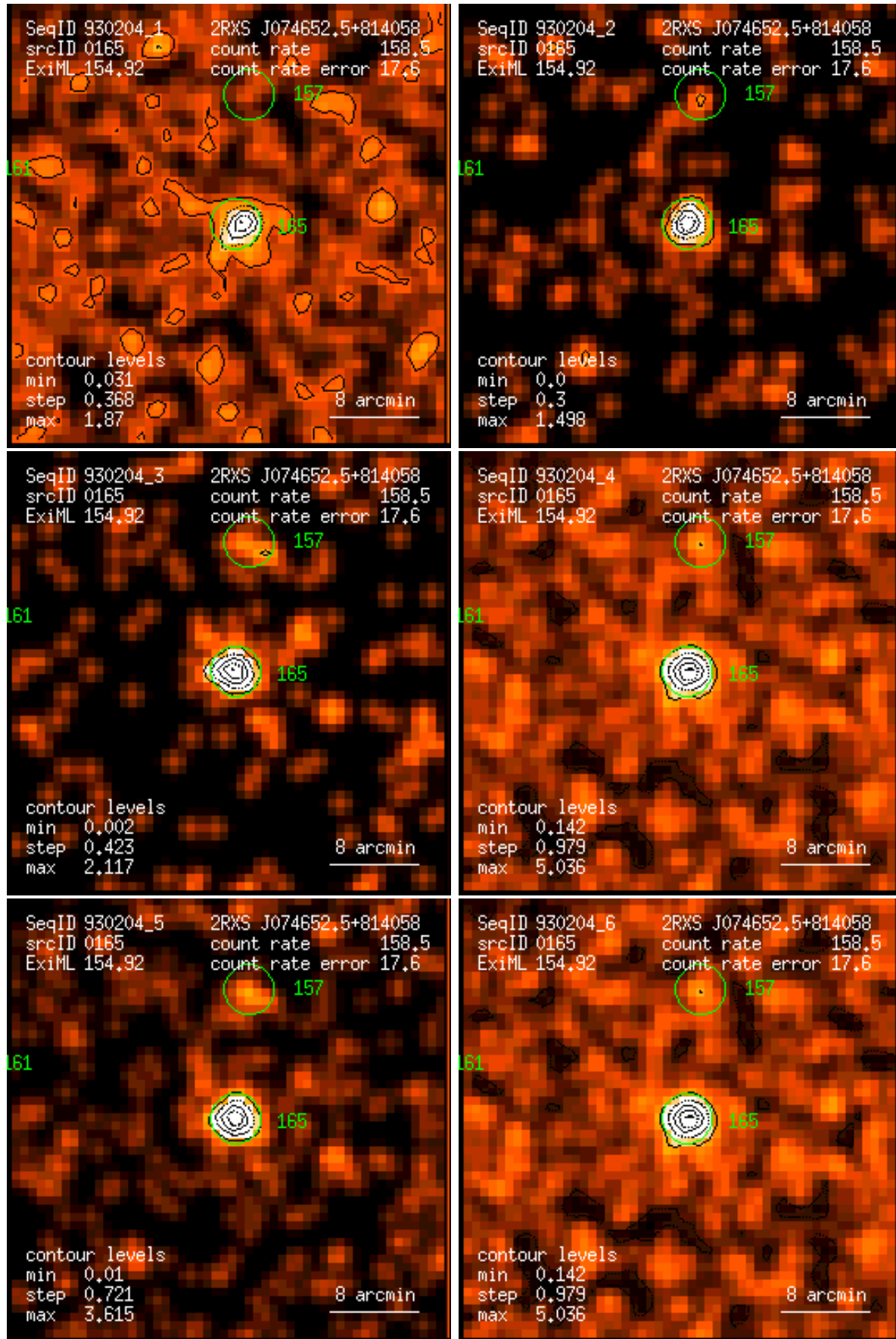
Figure 165: RASS 930204: detection 0165: band rate images, Gaussian filter: (1) PSPC channels 11 – 41, (2) 52 – 90, (3) 91 – 201, (4) 11 – 235, (5) 52 – 201, (6) 11 – 201. Broad band rates in counts/ks. Band rate contour levels in counts/ks/arcmin 2 .
