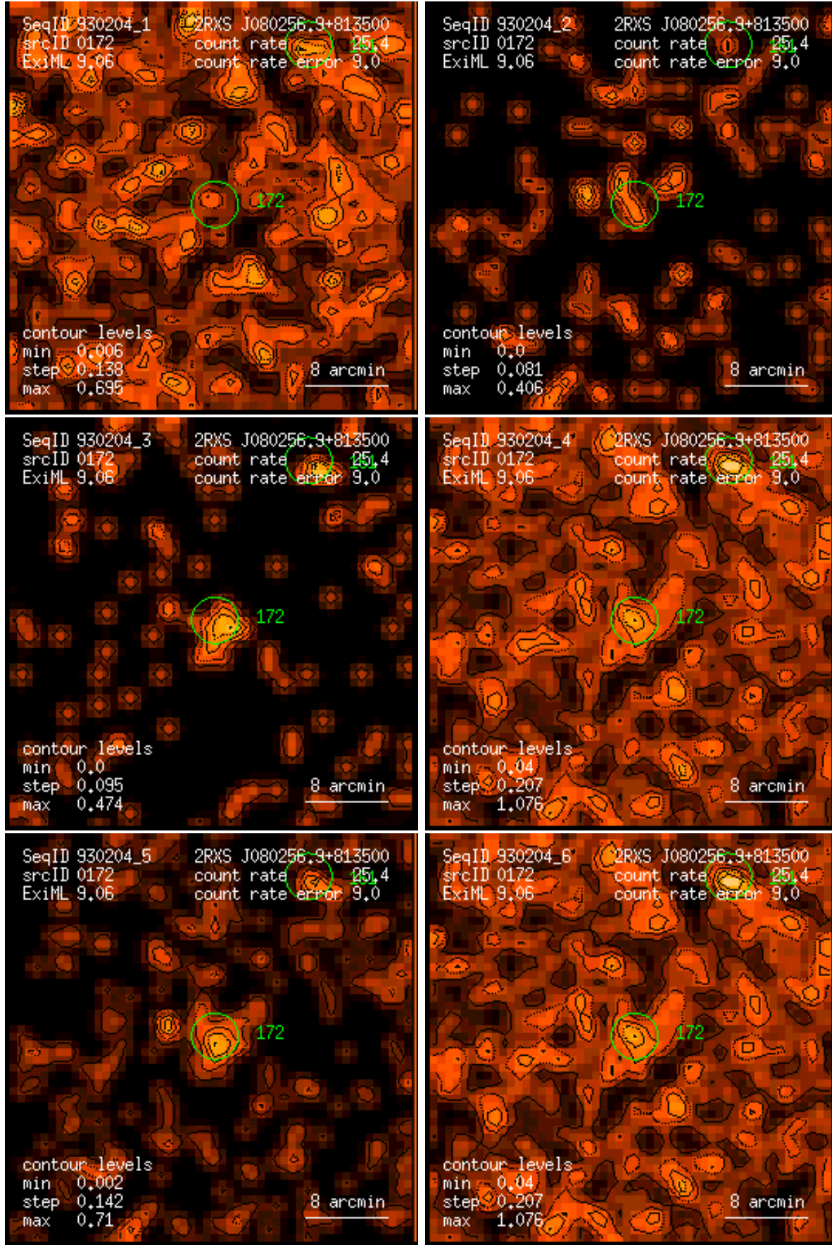
Figure 172: RASS 930204: detection 0172: band rate images, Gaussian filter: (1) PSPC channels 11 – 41, (2) 52 – 90, (3) 91 – 201, (4) 11 – 235, (5) 52 – 201, (6) 11 – 201. Broad band rates in counts/ks. Band rate contour levels in counts/ks/arcmin 2 .
