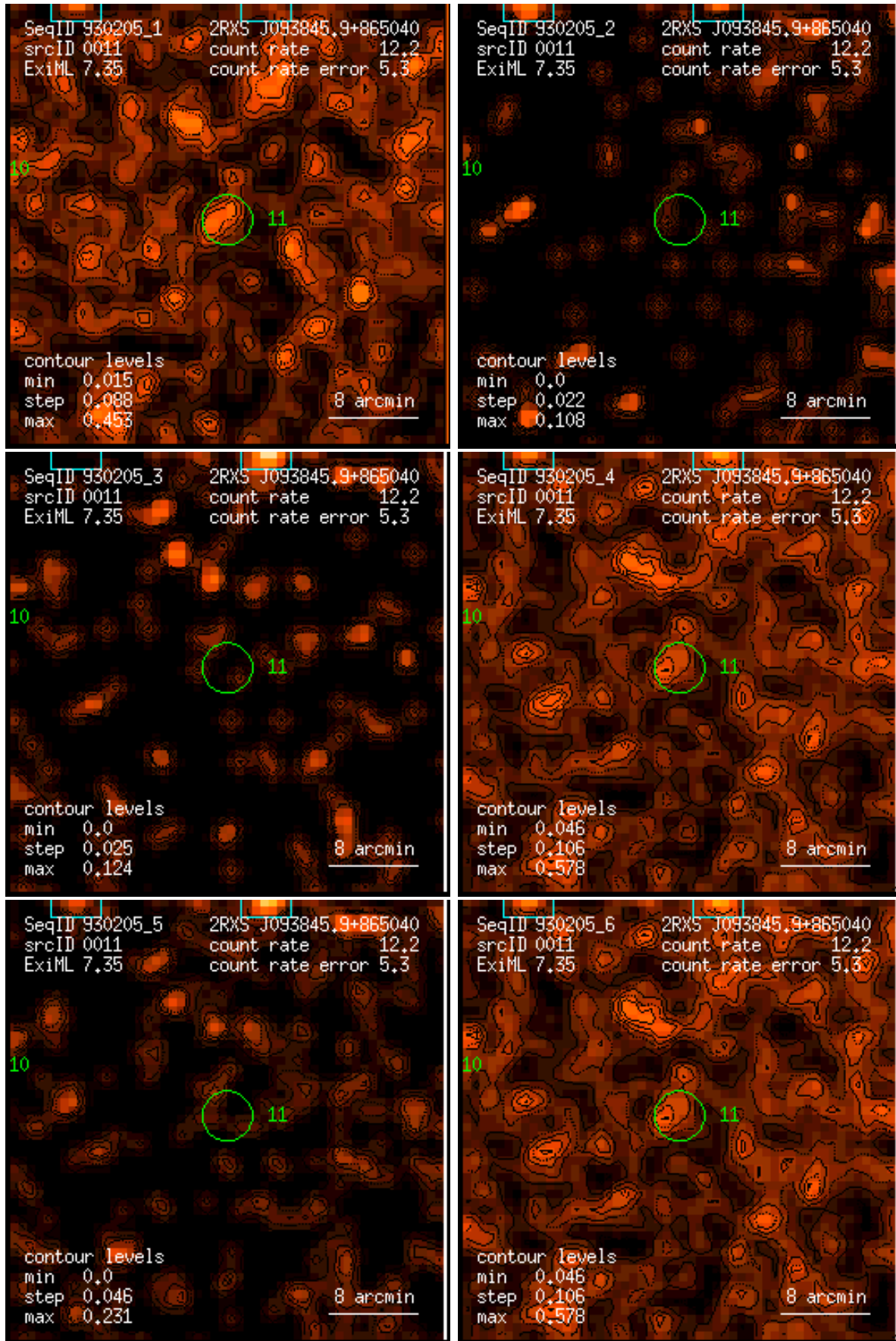
Figure 11: RASS 930205: detection 0011: band rate images, Gaussian filter: (1) PSPC channels 11 – 41, (2) 52 – 90, (3) 91 – 201, (4) 11 – 235, (5) 52 – 201, (6) 11 – 201. Broad band rates in counts/ks. Band rate contour levels in counts/ks/arcmin 2 .
