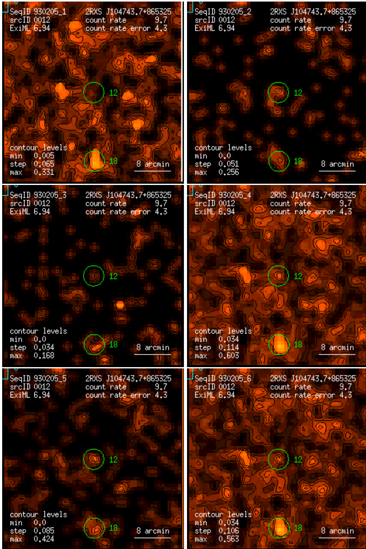
Figure 12: RASS 930205: detection 0012: band rate images, Gaussian filter: (1) PSPC channels 11 – 41, (2) 52 – 90, (3) 91 – 201, (4) 11 – 235, (5) 52 – 201, (6) 11 – 201. Broad band rates in counts/ks. Band rate contour levels in counts/ks/arcmin 2 .
