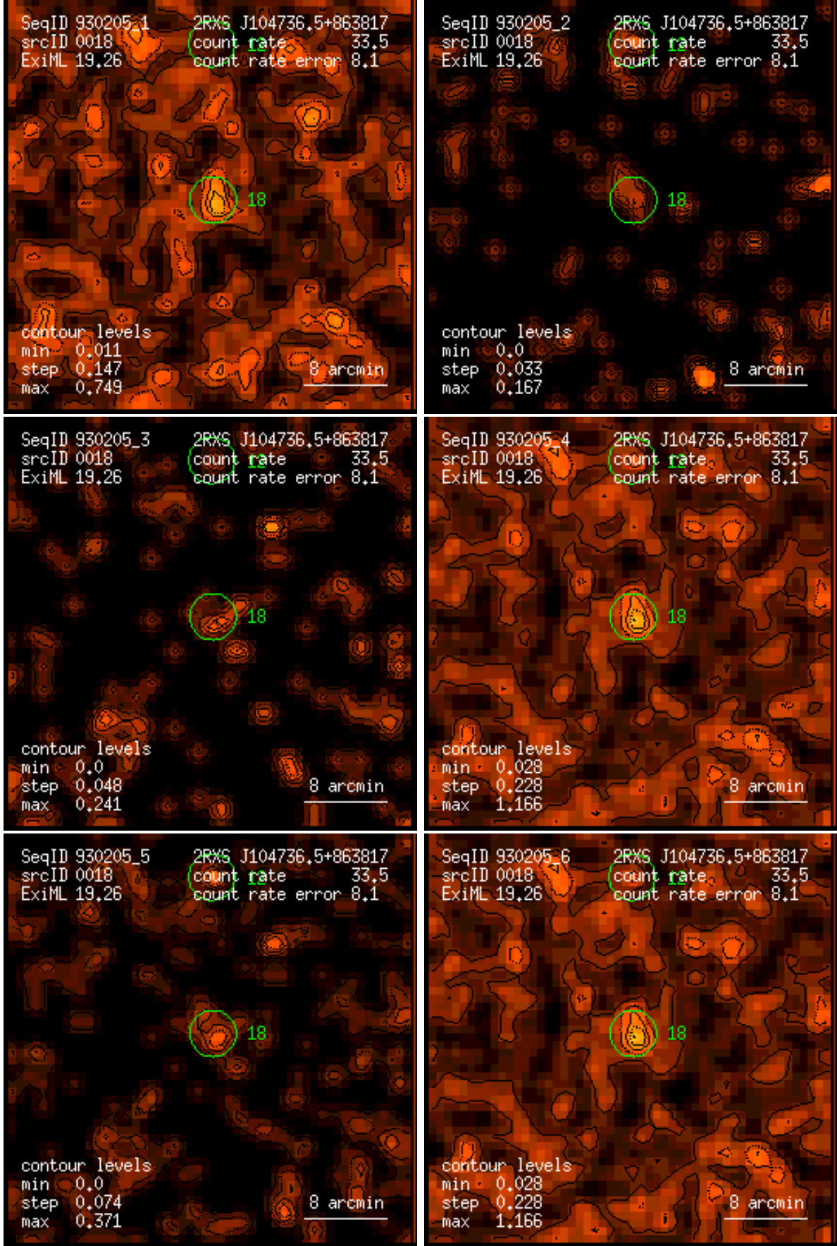
Figure 18: RASS 930205: detection 0018: band rate images, Gaussian filter: (1) PSPC channels 11 – 41, (2) 52 – 90, (3) 91 – 201, (4) 11 – 235, (5) 52 – 201, (6) 11 – 201. Broad band rates in counts/ks. Band rate contour levels in counts/ks/arcmin 2 .
