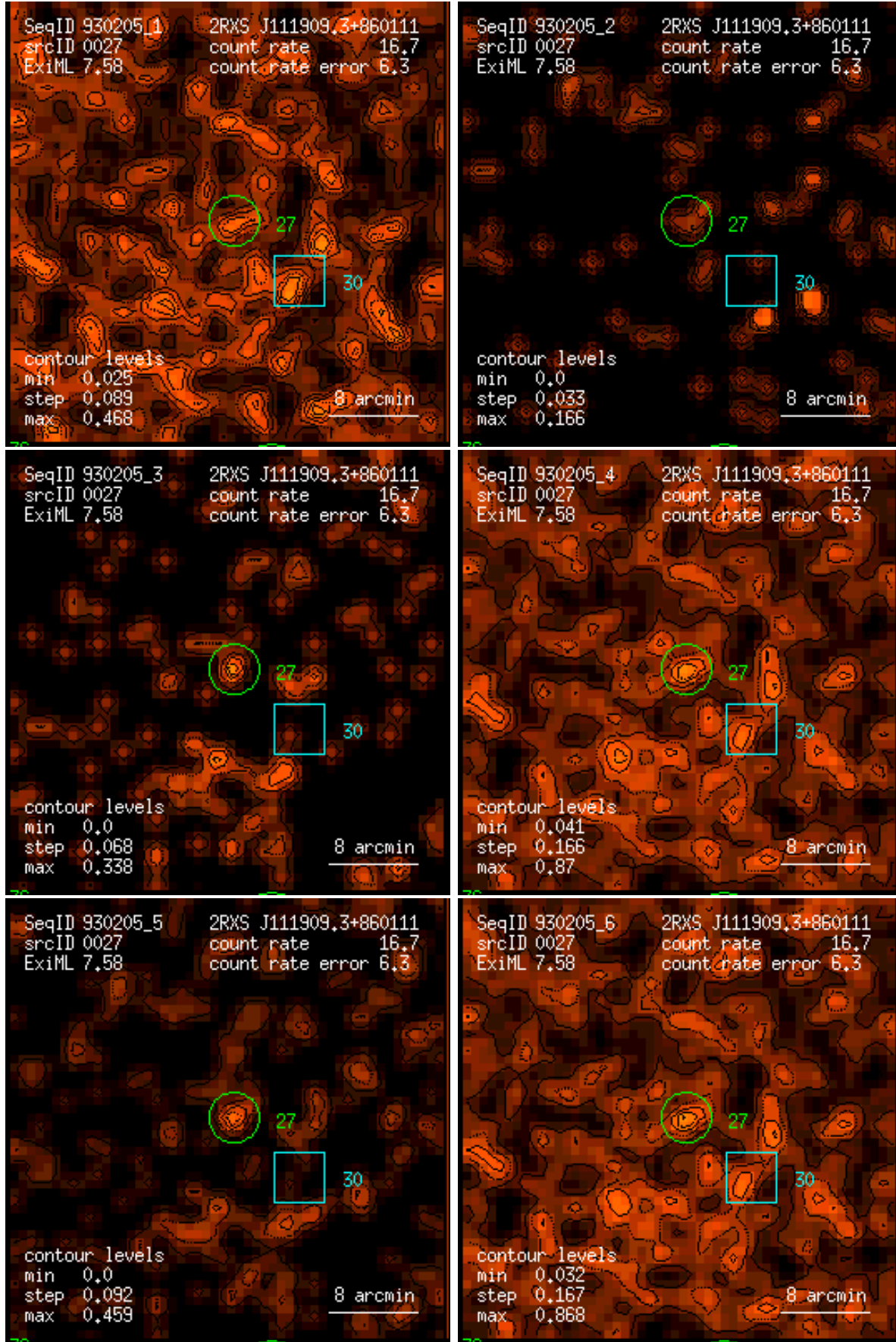
Figure 27: RASS 930205: detection 0027: band rate images, Gaussian filter: (1) PSPC channels 11 – 41, (2) 52 – 90, (3) 91 – 201, (4) 11 – 235, (5) 52 – 201, (6) 11 – 201. Broad band rates in counts/ks. Band rate contour levels in counts/ks/arcmin 2 .
