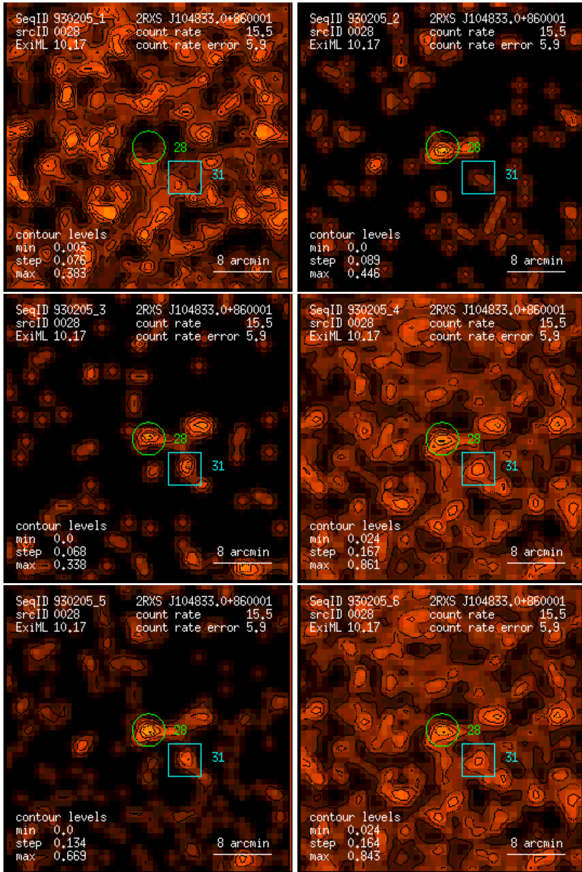
Figure 28: RASS 930205: detection 0028: band rate images, Gaussian filter: (1) PSPC channels 11 – 41, (2) 52 – 90, (3) 91 – 201, (4) 11 – 235, (5) 52 – 201, (6) 11 – 201. Broad band rates in counts/ks. Band rate contour levels in counts/ks/arcmin 2 .
