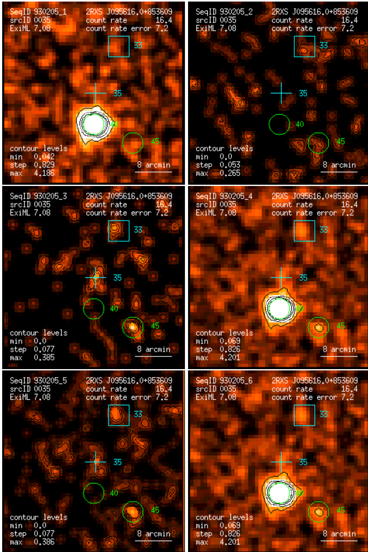
Figure 35: RASS 930205: detection 0035: band rate images, Gaussian filter: (1) PSPC channels 11 – 41, (2) 52 – 90, (3) 91 – 201, (4) 11 – 235, (5) 52 – 201, (6) 11 – 201. Broad band rates in counts/ks. Band rate contour levels in counts/ks/arcmin 2 .
