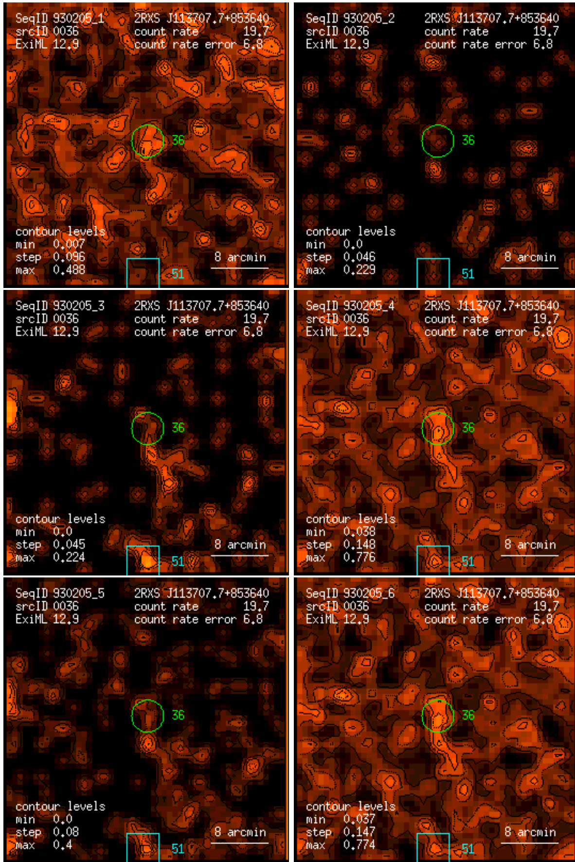
Figure 36: RASS 930205: detection 0036: band rate images, Gaussian filter: (1) PSPC channels 11 – 41, (2) 52 – 90, (3) 91 – 201, (4) 11 – 235, (5) 52 – 201, (6) 11 – 201. Broad band rates in counts/ks. Band rate contour levels in counts/ks/arcmin 2 .
