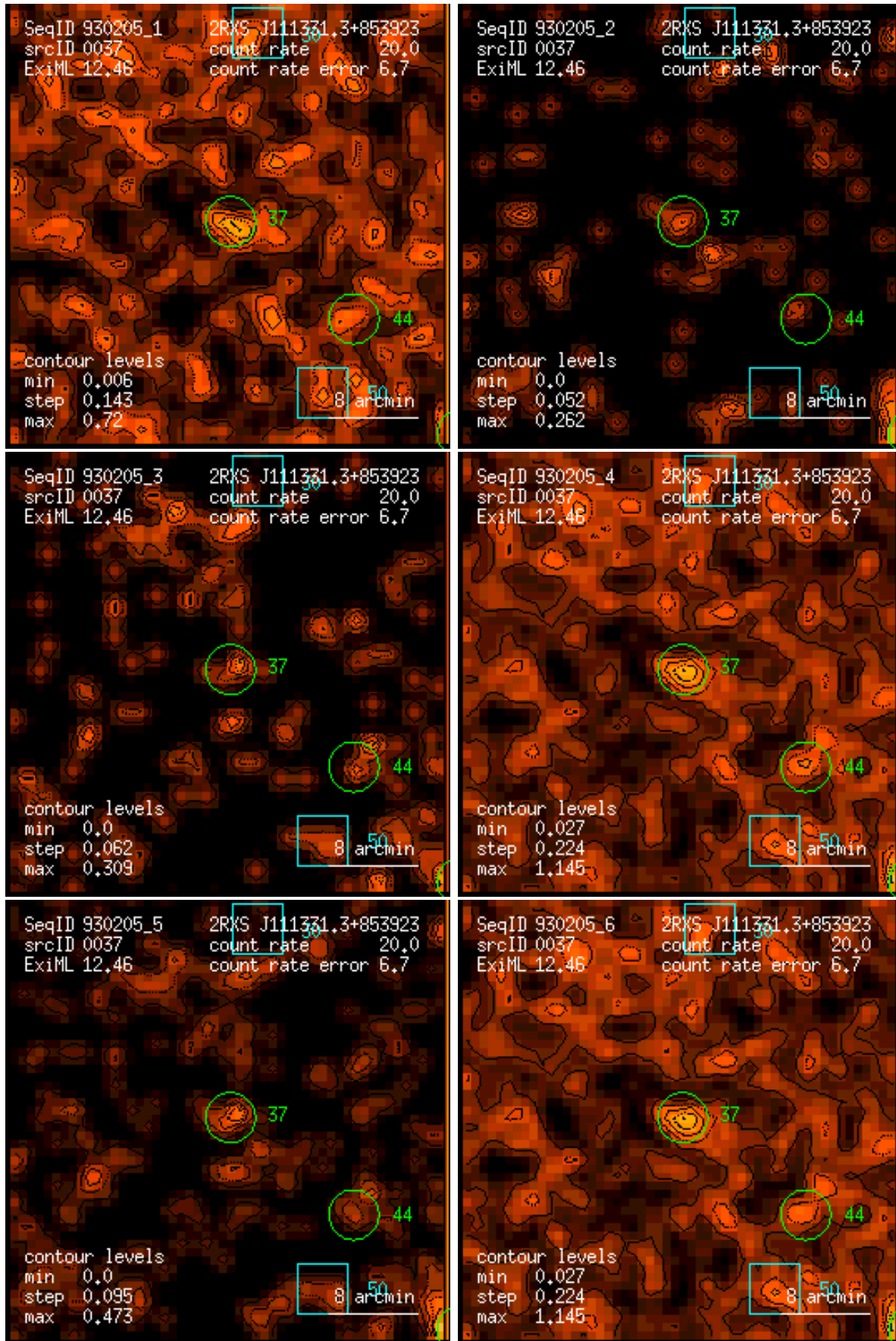
Figure 37: RASS 930205: detection 0037: band rate images, Gaussian filter: (1) PSPC channels 11 – 41, (2) 52 – 90, (3) 91 – 201, (4) 11 – 235, (5) 52 – 201, (6) 11 – 201. Broad band rates in counts/ks. Band rate contour levels in counts/ks/arcmin 2 .
