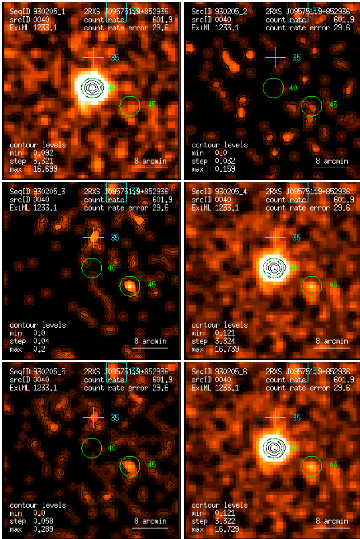
Figure 40: RASS 930205: detection 0040: band rate images, Gaussian filter: (1) PSPC channels 11 – 41, (2) 52 – 90, (3) 91 – 201, (4) 11 – 235, (5) 52 – 201, (6) 11 – 201. Broad band rates in counts/ks. Band rate contour levels in counts/ks/arcmin 2 .
