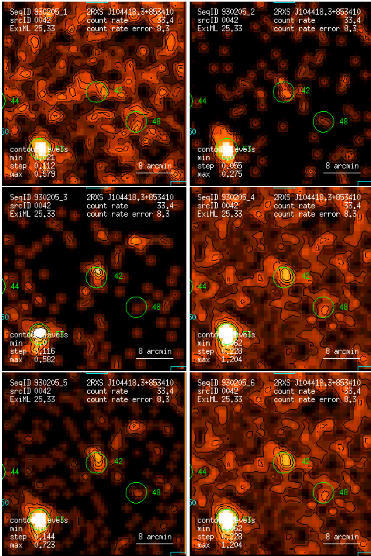
Figure 42: RASS 930205: detection 0042: band rate images, Gaussian filter: (1) PSPC channels 11 – 41, (2) 52 – 90, (3) 91 – 201, (4) 11 – 235, (5) 52 – 201, (6) 11 – 201. Broad band rates in counts/ks. Band rate contour levels in counts/ks/arcmin 2 .
