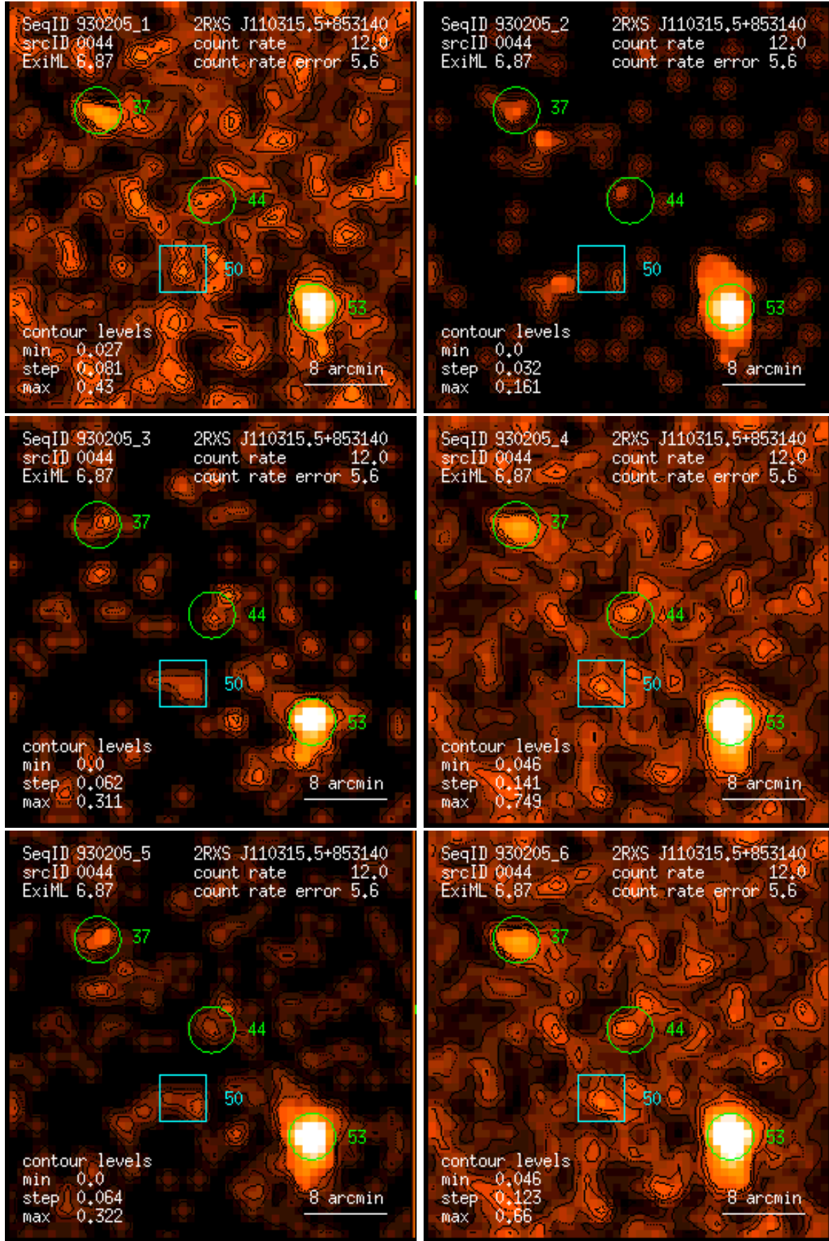
Figure 44: RASS 930205: detection 0044: band rate images, Gaussian filter: (1) PSPC channels 11 – 41, (2) 52 – 90, (3) 91 – 201, (4) 11 – 235, (5) 52 – 201, (6) 11 – 201. Broad band rates in counts/ks. Band rate contour levels in counts/ks/arcmin 2 .
