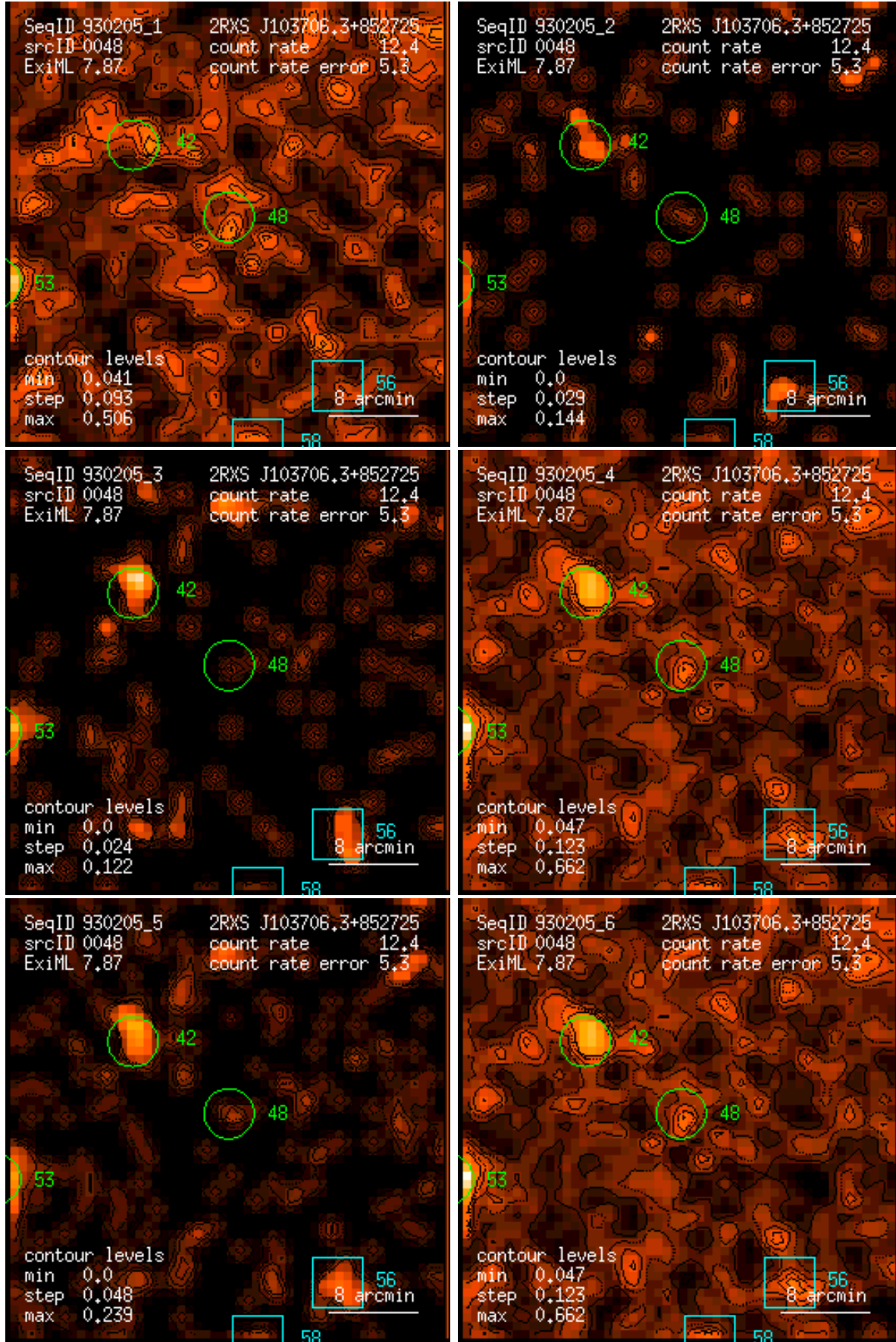
Figure 48: RASS 930205: detection 0048: band rate images, Gaussian filter: (1) PSPC channels 11 – 41, (2) 52 – 90, (3) 91 – 201, (4) 11 – 235, (5) 52 – 201, (6) 11 – 201. Broad band rates in counts/ks. Band rate contour levels in counts/ks/arcmin 2 .
