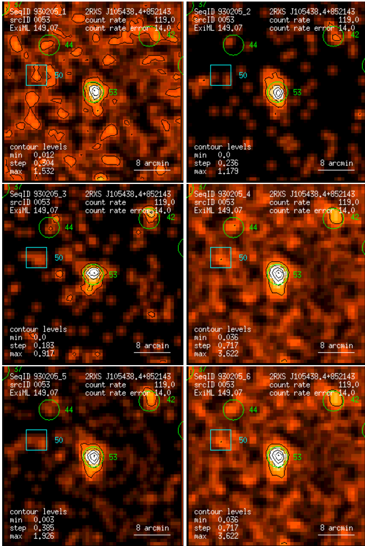
Figure 53: RASS 930205: detection 0053: band rate images, Gaussian filter: (1) PSPC channels 11 – 41, (2) 52 – 90, (3) 91 – 201, (4) 11 – 235, (5) 52 – 201, (6) 11 – 201. Broad band rates in counts/ks. Band rate contour levels in counts/ks/arcmin 2 .
