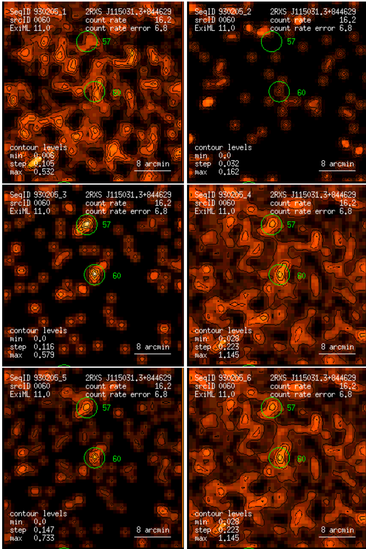
Figure 60: RASS 930205: detection 0060: band rate images, Gaussian filter: (1) PSPC channels 11 – 41, (2) 52 – 90, (3) 91 – 201, (4) 11 – 235, (5) 52 – 201, (6) 11 – 201. Broad band rates in counts/ks. Band rate contour levels in counts/ks/arcmin 2 .
