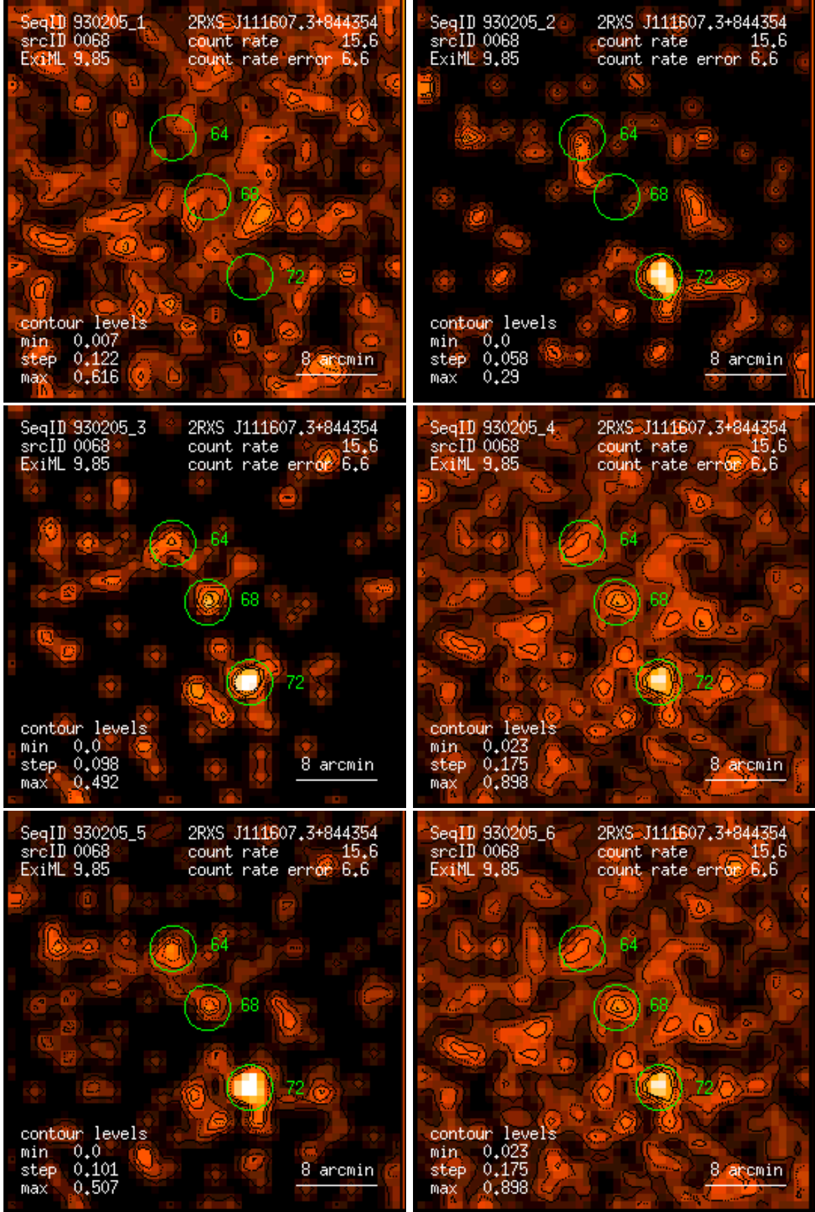
Figure 68: RASS 930205: detection 0068: band rate images, Gaussian filter: (1) PSPC channels 11 – 41, (2) 52 – 90, (3) 91 – 201, (4) 11 – 235, (5) 52 – 201, (6) 11 – 201. Broad band rates in counts/ks. Band rate contour levels in counts/ks/arcmin 2 .
