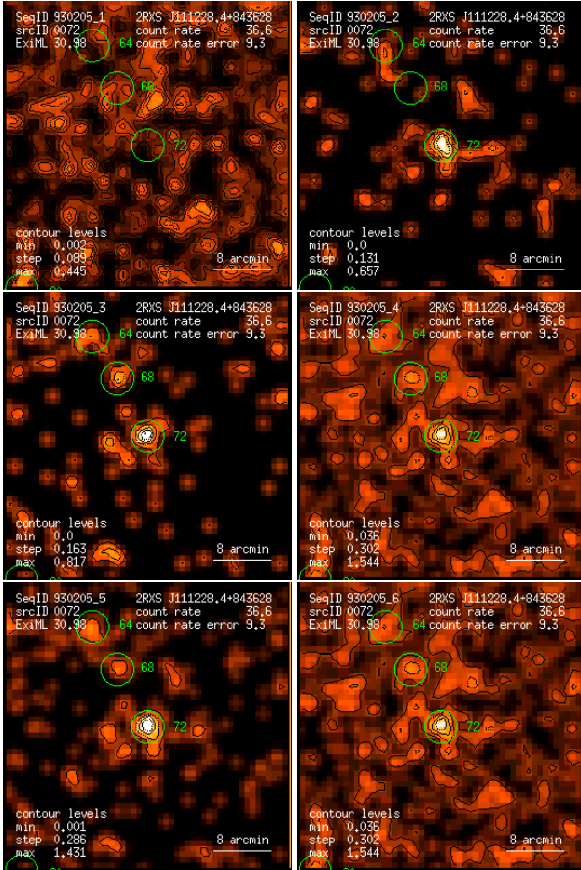
Figure 72: RASS 930205: detection 0072: band rate images, Gaussian filter: (1) PSPC channels 11 – 41, (2) 52 – 90, (3) 91 – 201, (4) 11 – 235, (5) 52 – 201, (6) 11 – 201. Broad band rates in counts/ks. Band rate contour levels in counts/ks/arcmin 2 .
