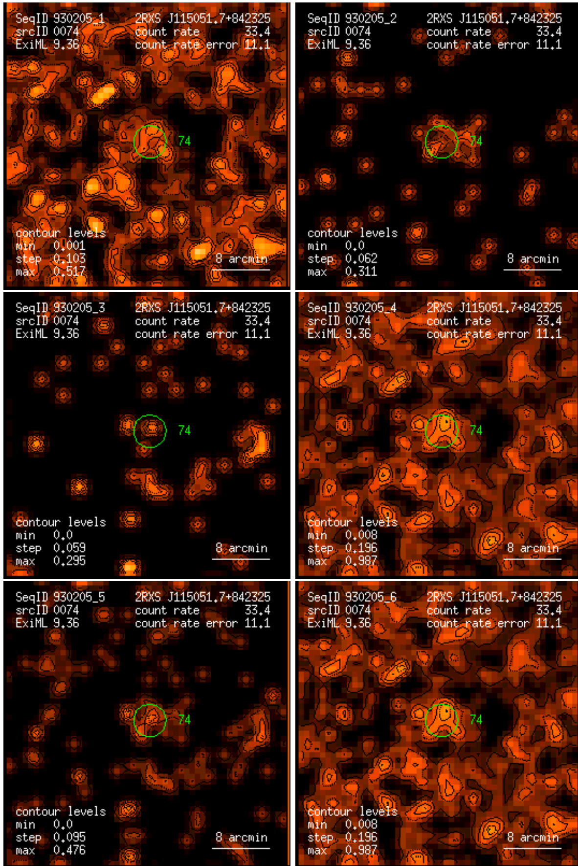
Figure 74: RASS 930205: detection 0074: band rate images, Gaussian filter: (1) PSPC channels 11 – 41, (2) 52 – 90, (3) 91 – 201, (4) 11 – 235, (5) 52 – 201, (6) 11 – 201. Broad band rates in counts/ks. Band rate contour levels in counts/ks/arcmin 2 .
