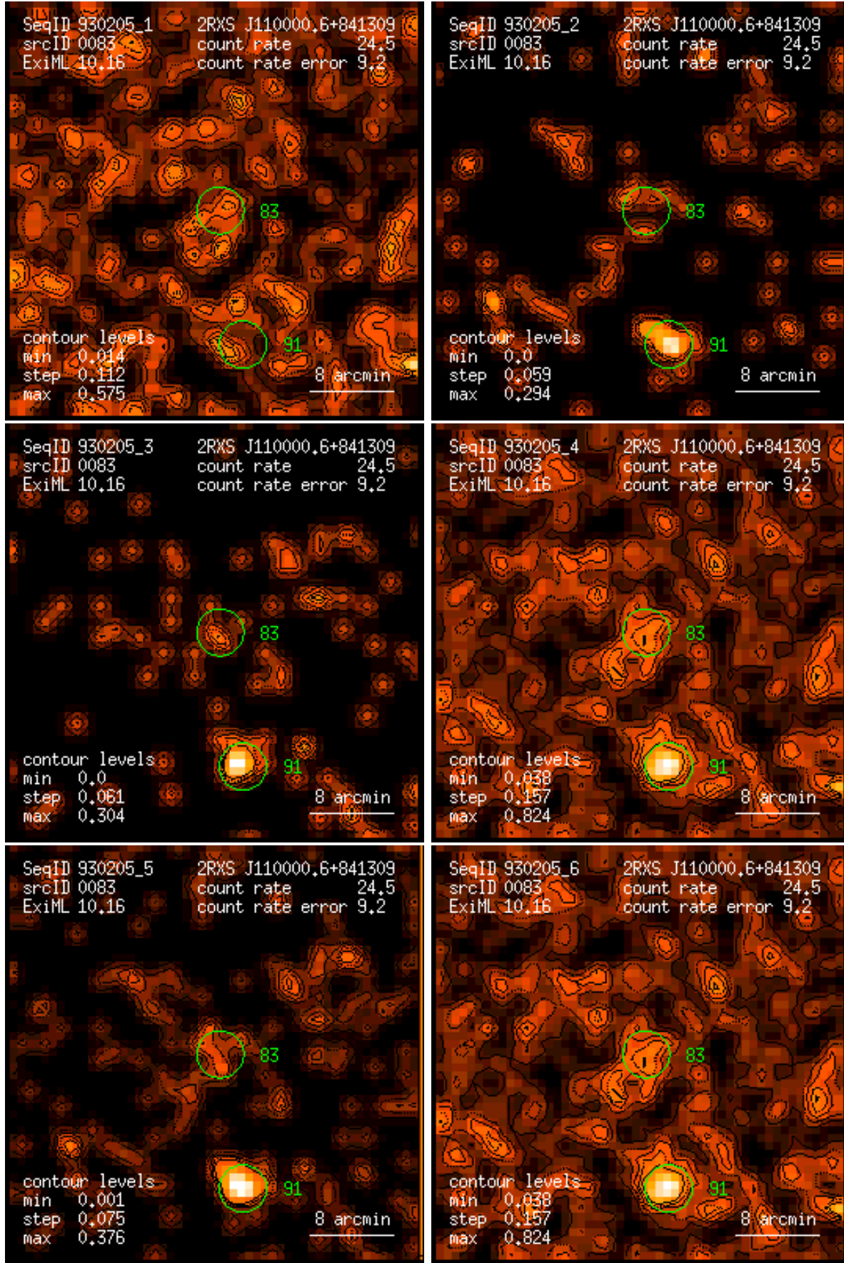
Figure 83: RASS 930205: detection 0083: band rate images, Gaussian filter: (1) PSPC channels 11 – 41, (2) 52 – 90, (3) 91 – 201, (4) 11 – 235, (5) 52 – 201, (6) 11 – 201. Broad band rates in counts/ks. Band rate contour levels in counts/ks/arcmin 2 .
