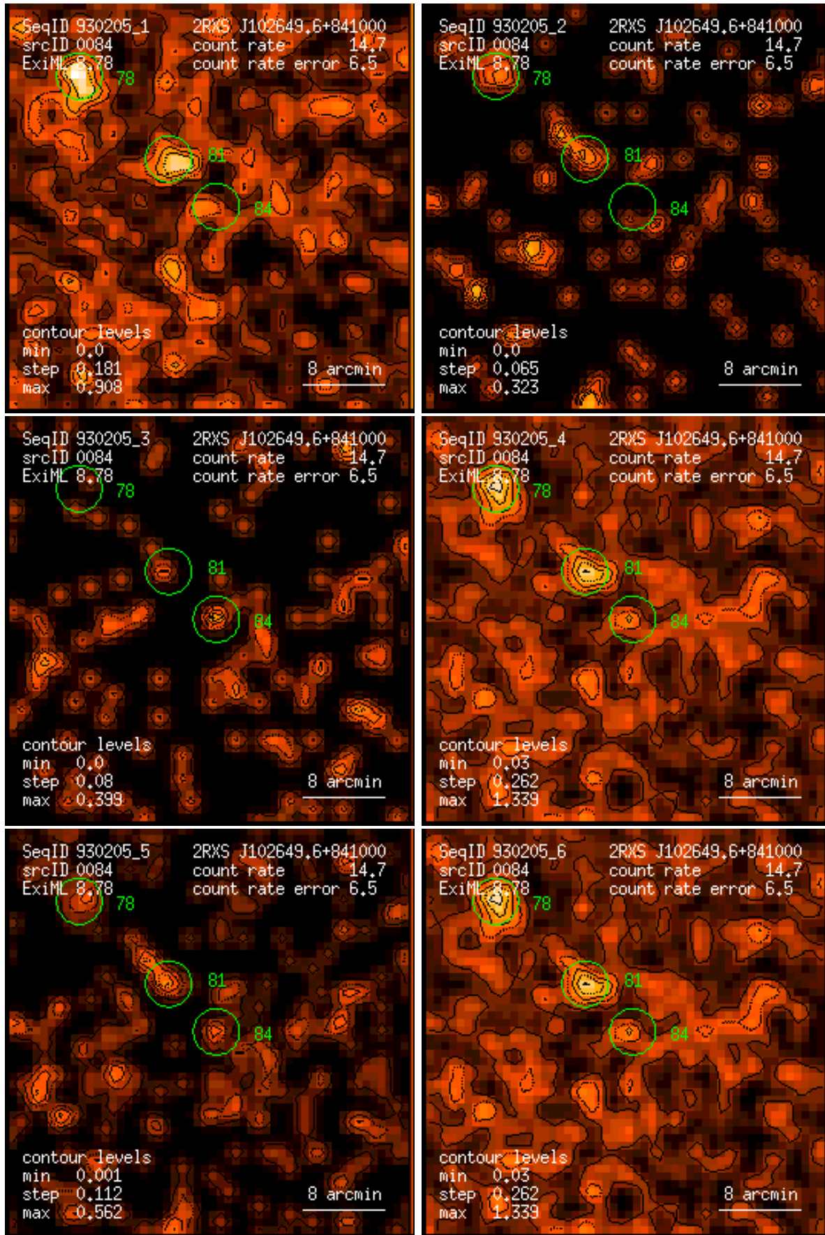
Figure 84: RASS 930205: detection 0084: band rate images, Gaussian filter: (1) PSPC channels 11 – 41, (2) 52 – 90, (3) 91 – 201, (4) 11 – 235, (5) 52 – 201, (6) 11 – 201. Broad band rates in counts/ks. Band rate contour levels in counts/ks/arcmin 2 .
