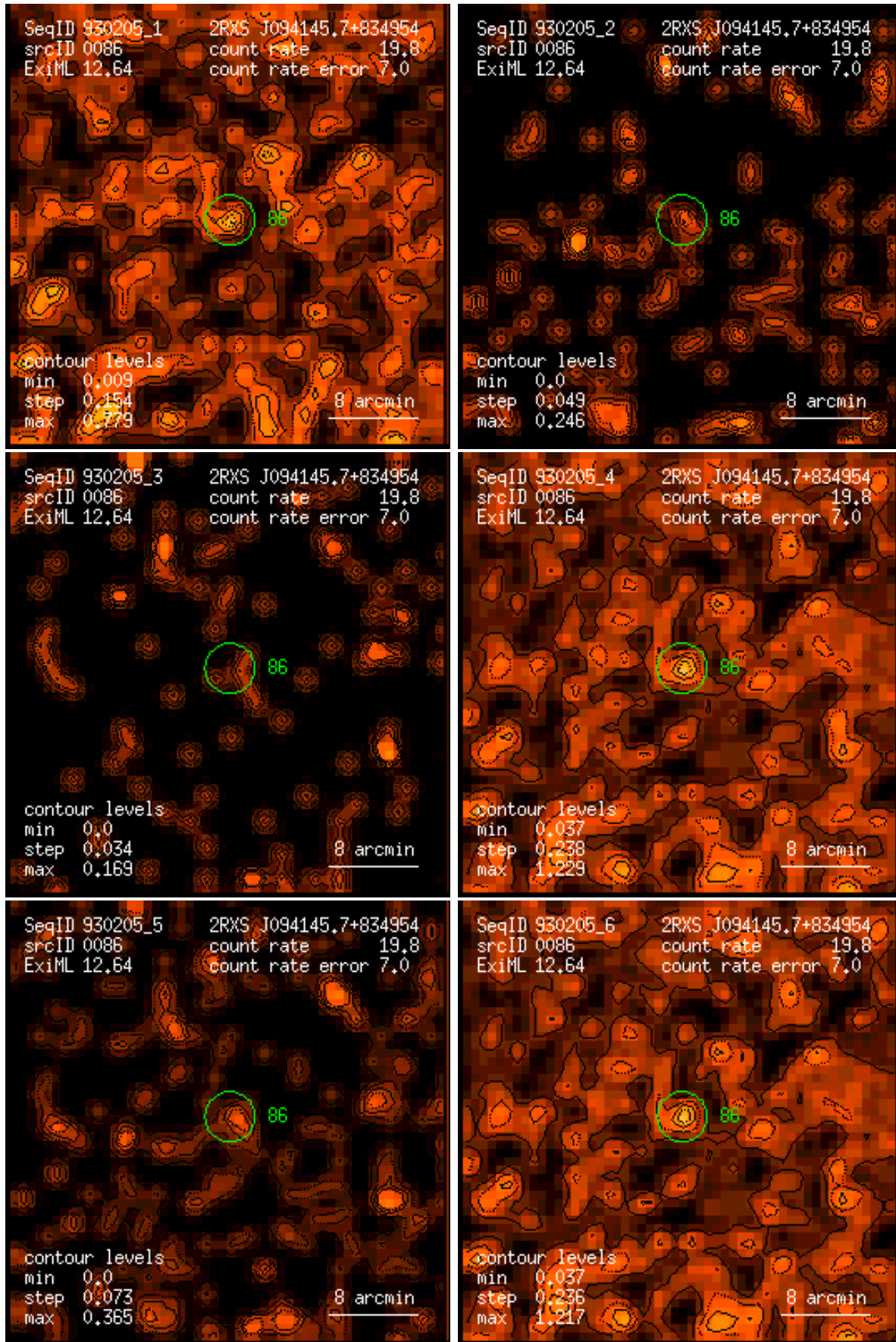
Figure 86: RASS 930205: detection 0086: band rate images, Gaussian filter: (1) PSPC channels 11 – 41, (2) 52 – 90, (3) 91 – 201, (4) 11 – 235, (5) 52 – 201, (6) 11 – 201. Broad band rates in counts/ks. Band rate contour levels in counts/ks/arcmin 2 .
