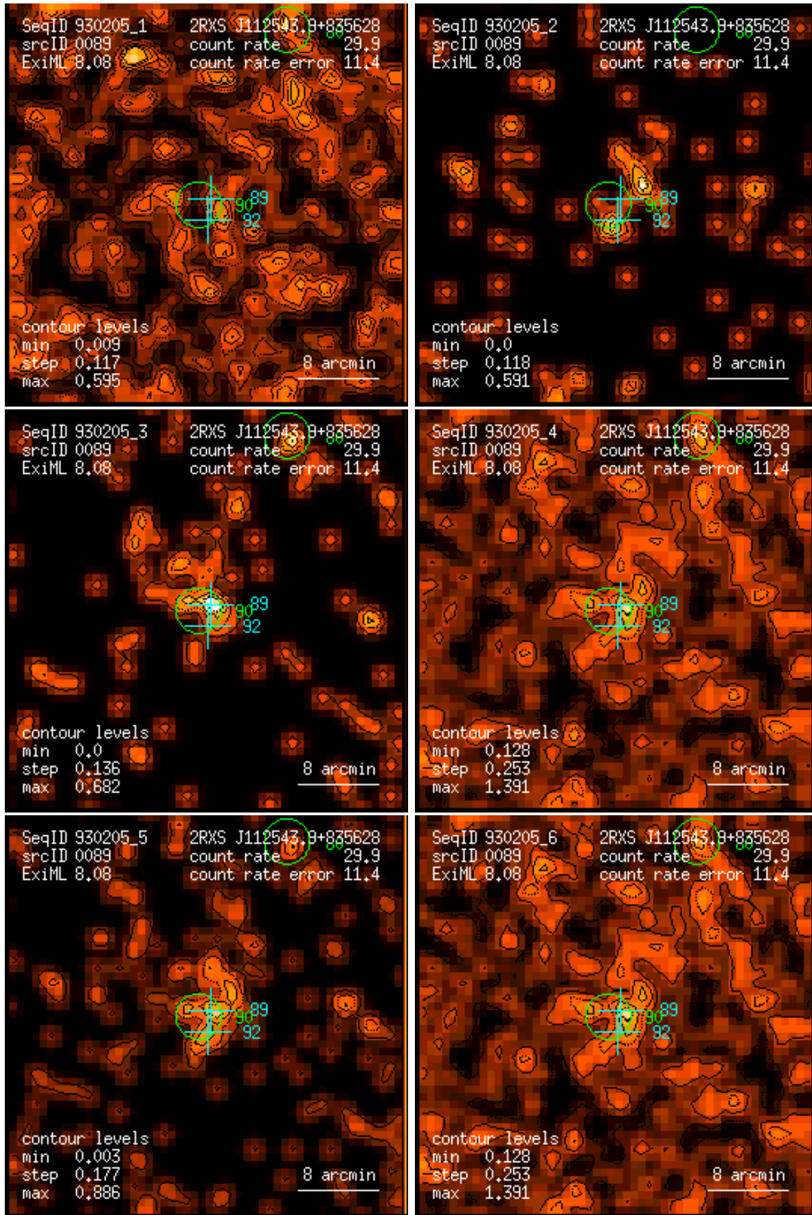
Figure 89: RASS 930205: detection 0089: band rate images, Gaussian filter: (1) PSPC channels 11 – 41, (2) 52 – 90, (3) 91 – 201, (4) 11 – 235, (5) 52 – 201, (6) 11 – 201. Broad band rates in counts/ks. Band rate contour levels in counts/ks/arcmin 2 .
