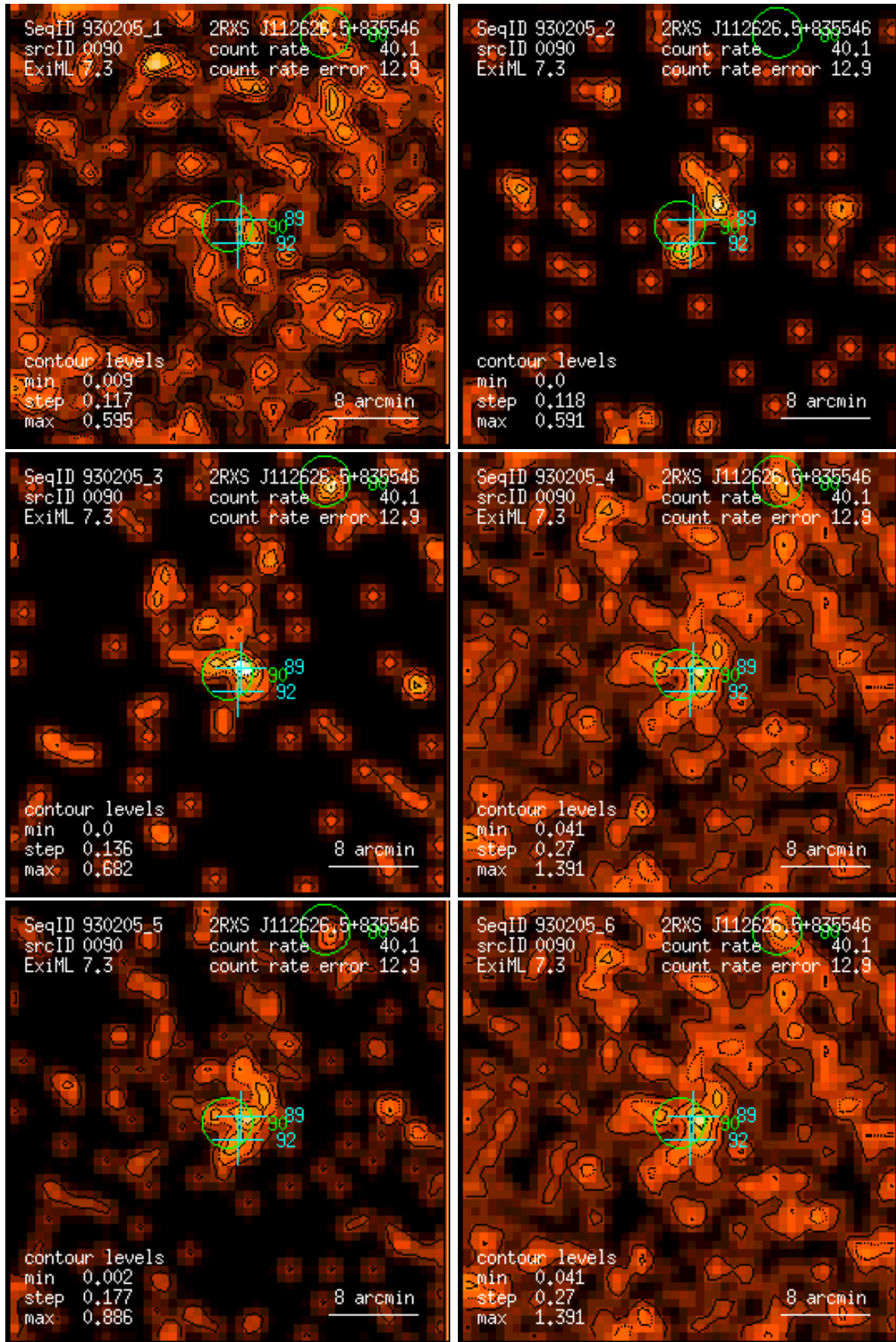
Figure 90: RASS 930205: detection 0090: band rate images, Gaussian filter: (1) PSPC channels 11 – 41, (2) 52 – 90, (3) 91 – 201, (4) 11 – 235, (5) 52 – 201, (6) 11 – 201. Broad band rates in counts/ks. Band rate contour levels in counts/ks/arcmin 2 .
