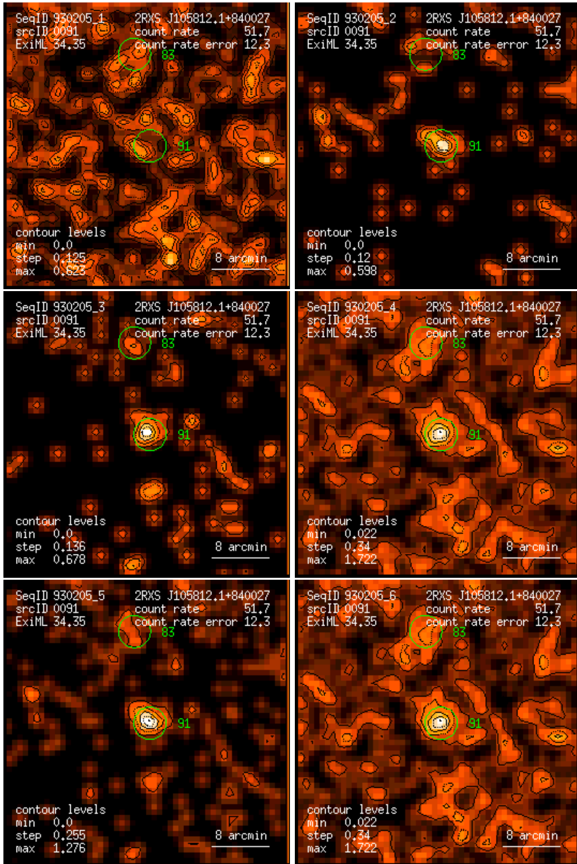
Figure 91: RASS 930205: detection 0091: band rate images, Gaussian filter: (1) PSPC channels 11 – 41, (2) 52 – 90, (3) 91 – 201, (4) 11 – 235, (5) 52 – 201, (6) 11 – 201. Broad band rates in counts/ks. Band rate contour levels in counts/ks/arcmin 2 .
